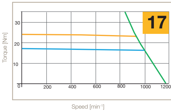
1000 min -1 400 V
