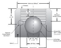
Port Dimensions: Parker X44 (Requires X44 Male Adapter to interface) Page 81
