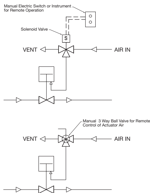
Fail Open - C1S Actuator shown
