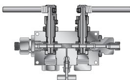
MADBB Series Double Block & Bleed Ball Valve Page 56
