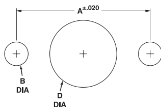
Needle Valve Panel Mount
