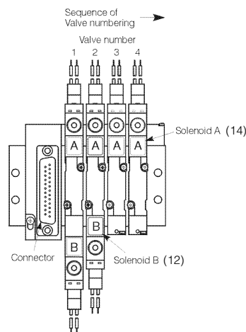
Valve and solenoid addresses
