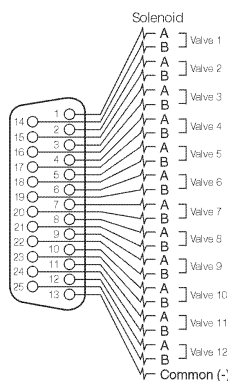
Pin map for Sub-D25 connector
