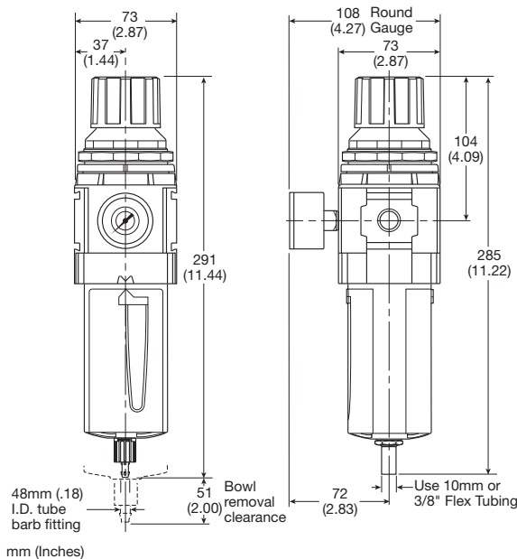
Manual Drain
