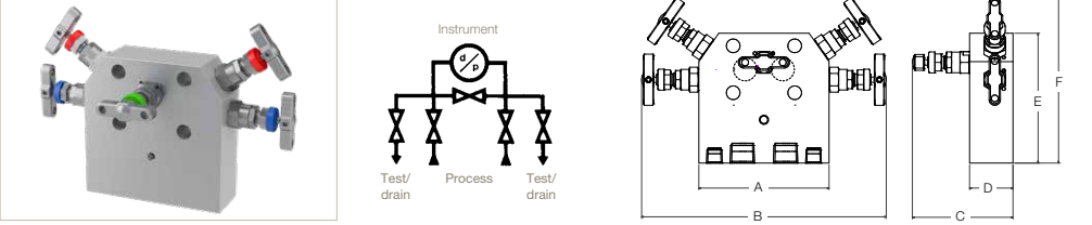
HD*5MCPEXT - Female threaded - NPT x Flanged
