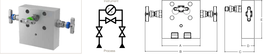
HD*3MCPEXT - Female threaded - NPT x Flanged
