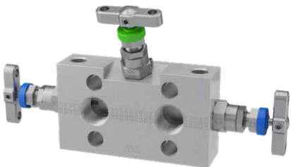
Example shown: 3-valve direct mount manifold with NPT connections and additional test/purge ports.
