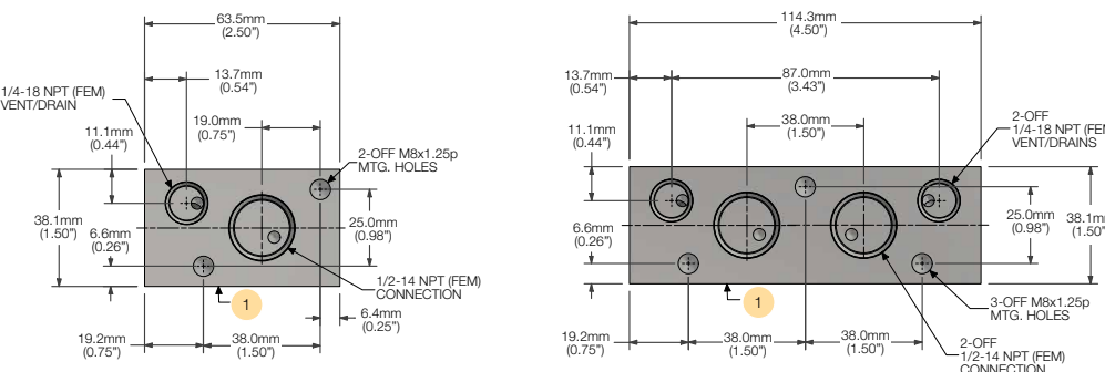
Manifold footprint for 2-valve manifolds. Example shown: HDS2EXT
