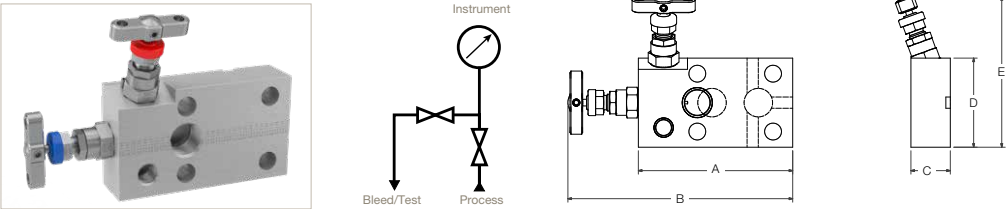
HD*2MCP - Female threaded - NPT x Flanged
