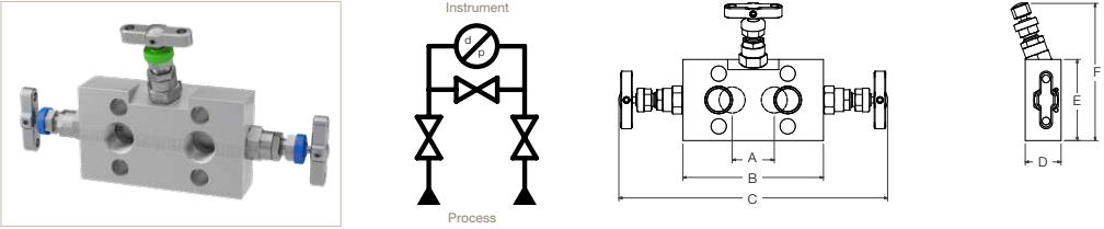
HD*3MCP - Female threaded - NPT x Flanged
