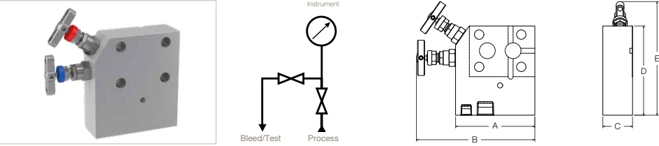
HD*2MCPEXT - Female threaded - NPT x Flanged
