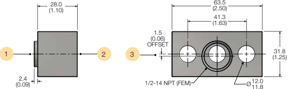
Example shown with traditional 1/2" NPT Fem. connection.
