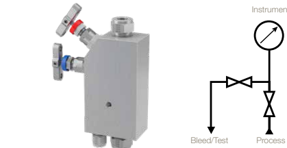
Example shown: 2-valve base connected manifold especially suited for use within enclosures, having Parker Superior Advantage fully integrated inverted style tube connections to inlet, outlet and vent/drain/bleed.
