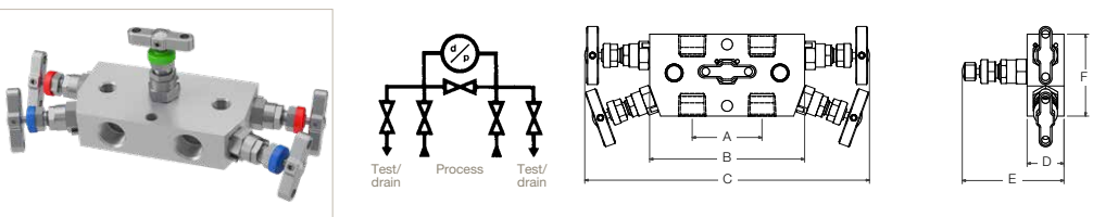
Example shown: 5-valve remote/line mount manifold featuring the Parker A-LOK® Superior Advantage Inverted integral tube fitting connections for the impulse line and NPT ported connections for the vent/ drains.
