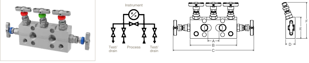
HD*5MCP - Female threaded - NPT x Flanged
