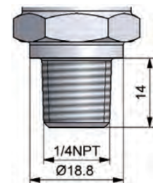
SCP03-xxx-x5-0x 1/4 NPT
