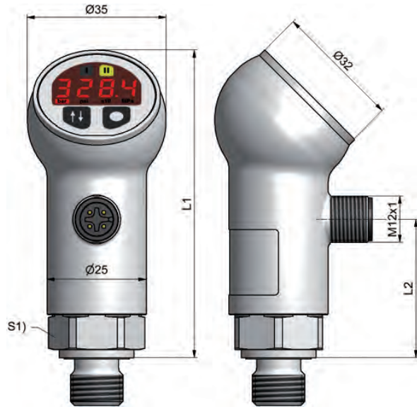
SCPSDi-xxx-xx-17
