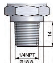
SCP03-xxx-x5-0x 1/4 NPT
