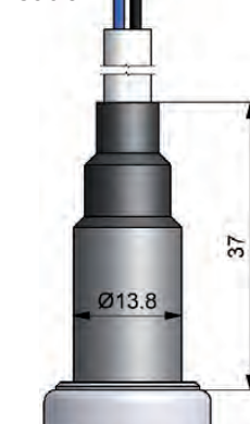
SCP03-xxx-x5-0x 1/4 NPT
