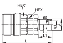
Male Thread 24° cone – DIN 2353 Bulkhead
