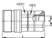
Female BSPP Thread – DIN 3852 Form Y
