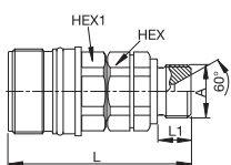
Male BSPP Thread – DIN 3852 Form B
