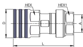
Female Thread - NPTF
