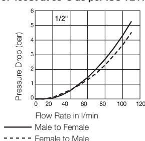
Flow Capacity with Oil with Viscosity of 43cSt at 38°C as per ISO 7241/2-2000
