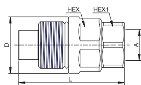
Female Thread - NPTF
