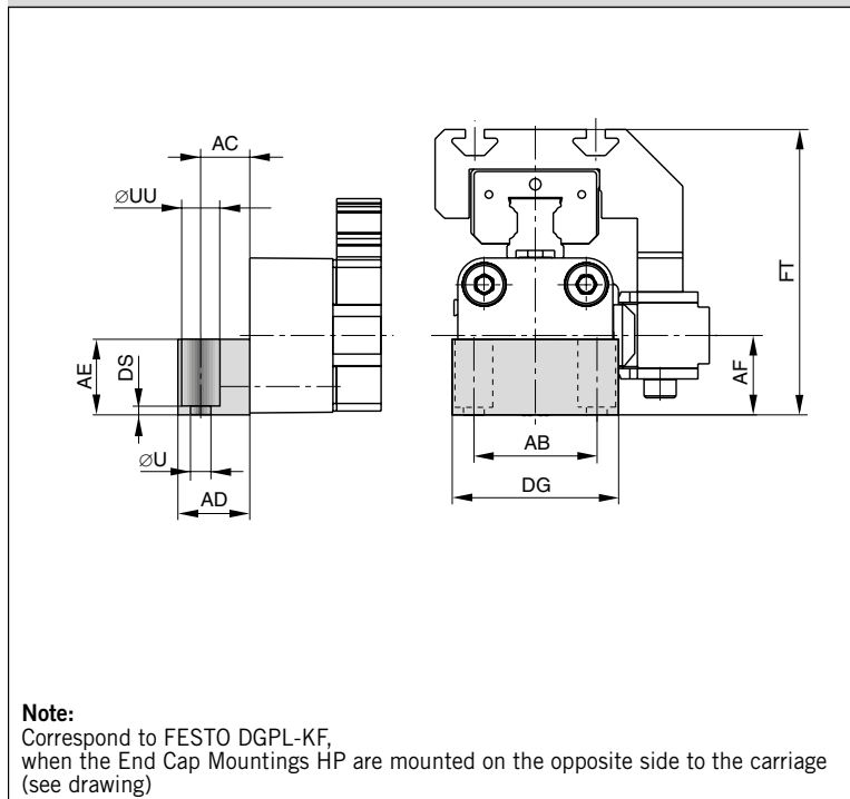
Series OSP-P KF25 to KF50: Type HP (Correspond to FESTO dimensions)
