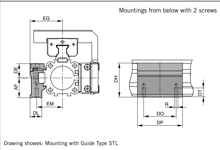
Dimension Table [mm] Mid-Section Support D1ST
