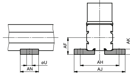
Series OSP-P16 to P80: Type E1 (Mounting from above / below using a cap screw)
