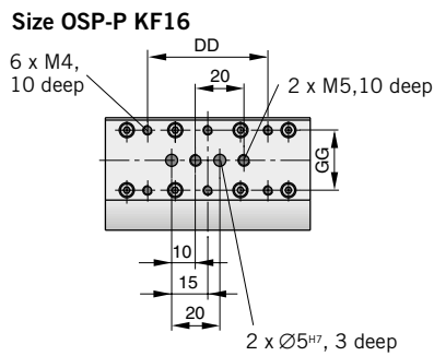
Dimension Table [mm] Series OSP-P KF16, KF25, KF32, KF40, KF50
