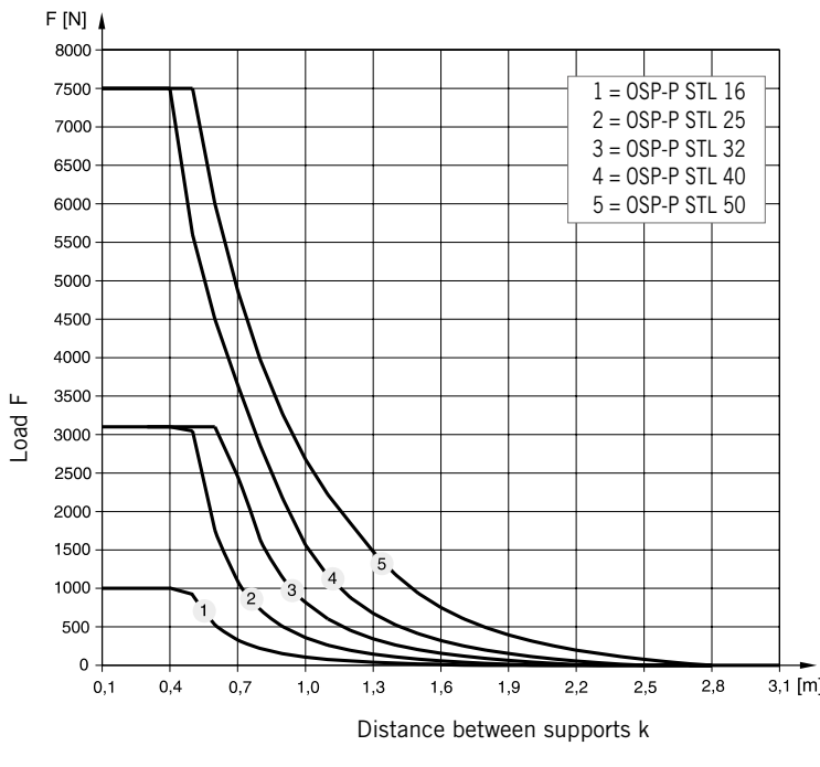
Loading 1 – Top carrier
