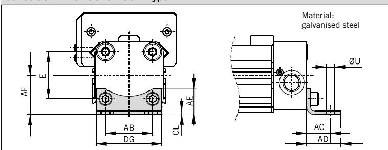
Series OSPP-BG40 and BG50: Type C1 (Supplied in pairs)
