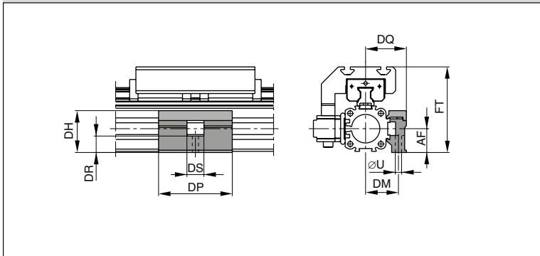
Series OSP-P KF25: Type MUP (Mounting over through holes)
