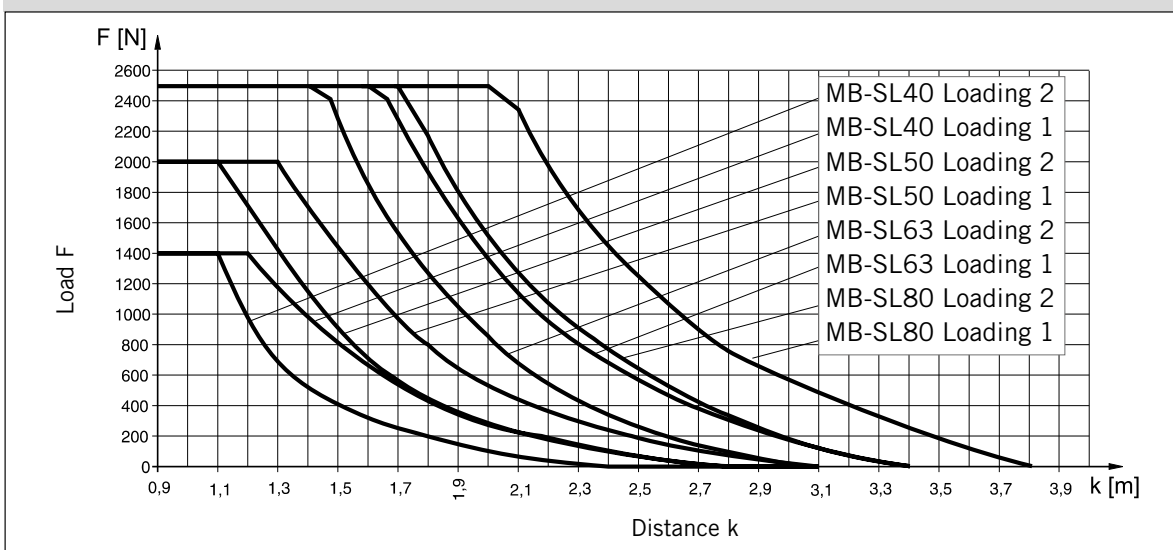
Permissible Unsupported Length MB-SL40, MB-SL50, MB-SL63 and MB-SL80
