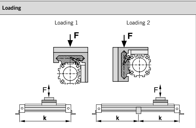
Permissible Unsupported Length MB-SL25, MB-SL32
