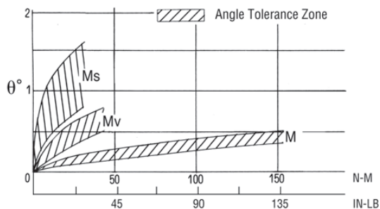
50 mm Bore
