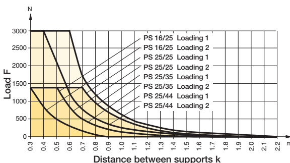
Permissible unsupported length: POWERSLIDE 16/25, 25/25, 25/35, 25/44mm bore
