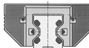
Full profile snap-on wiper
