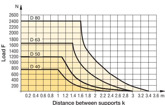
Basic cylinder 40 to 80mm bore mid-section supports
