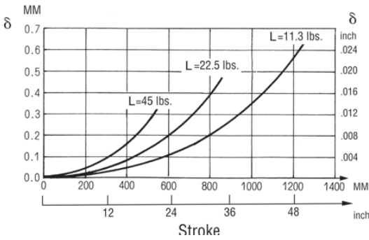
25 mm Bore
