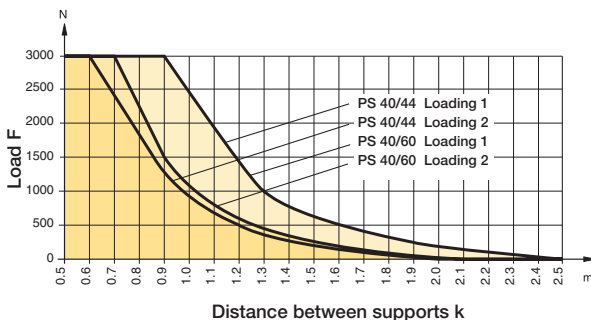
Permissible unsupported length: POWERSLIDE 40/44, 40/60mm bore
