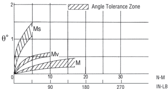
25 mm Bore
