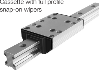
Full profile snap-on wiper
