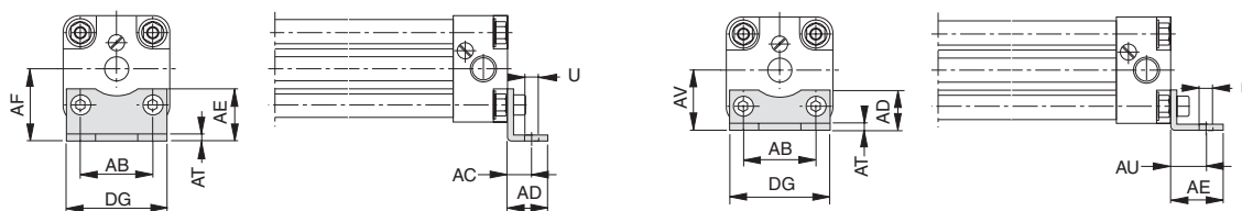
NR4 Mounting Bracket - Mtg. Style "A"
