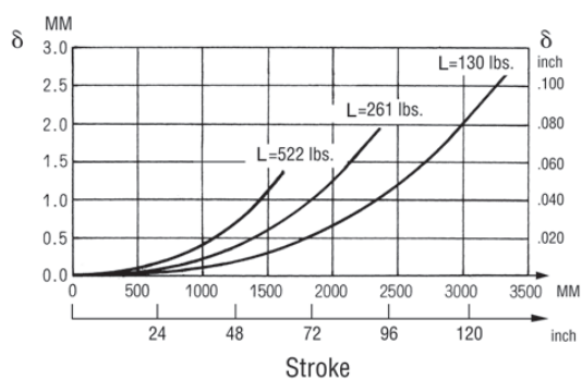
63 mm Bore
