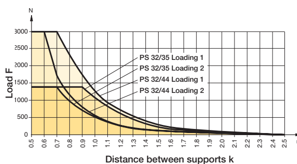
Permissible unsupported length: POWERSLIDE 2/35, 32/44mm bore
