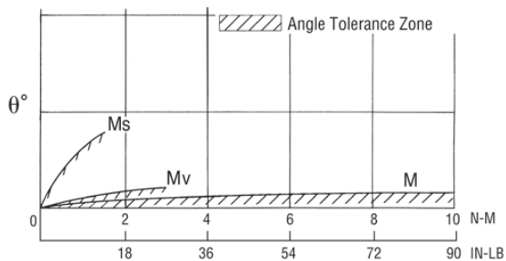
20 mm Bore
