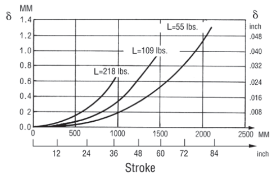
50 mm Bore
