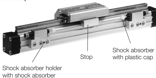
Arrangement with two variable stops
