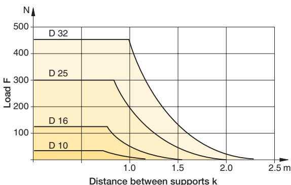
Basic cylinder 10 to 32mm bore mid-section supports
