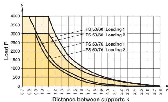
Permissible unsupported length: POWERSLIDE 50/60, 50/76mm bore
