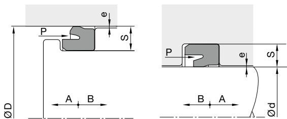
A = pushing B = pulling
