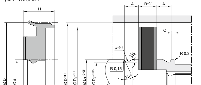
Type 1: D < 32 mm
