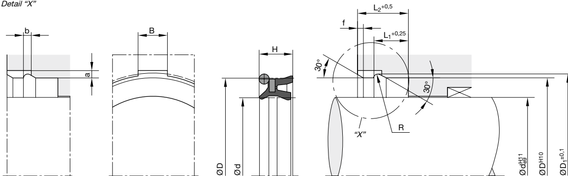
Detail "X"
