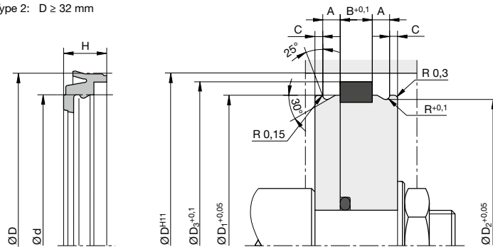
Type 2: D \geq 32 mm
