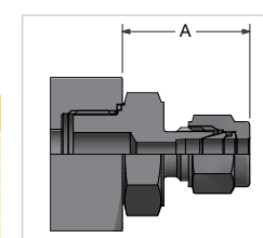
PTFree connect™ male connector (Code PFC)
