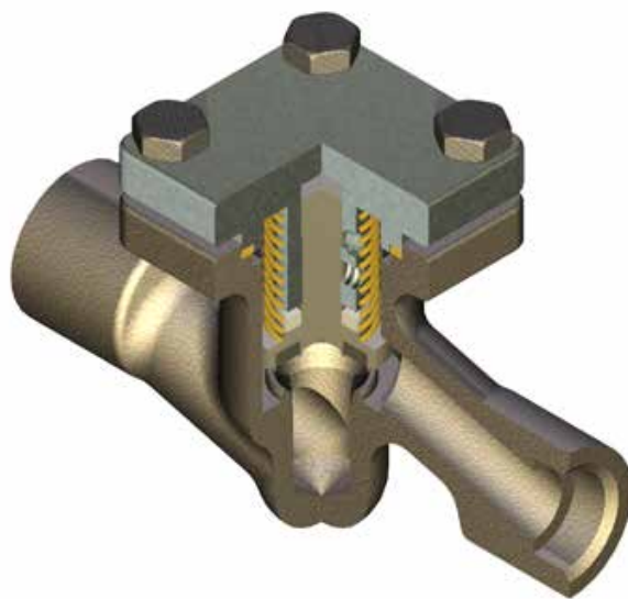
T51F-RUV/TF, DN25
