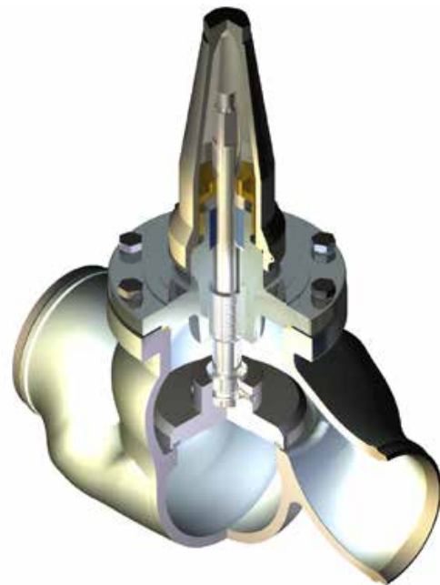
T5F, DN200
