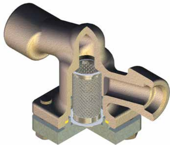
T51F-SS, DN25
