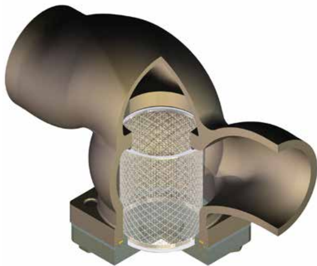
T5F-SS, DN100
