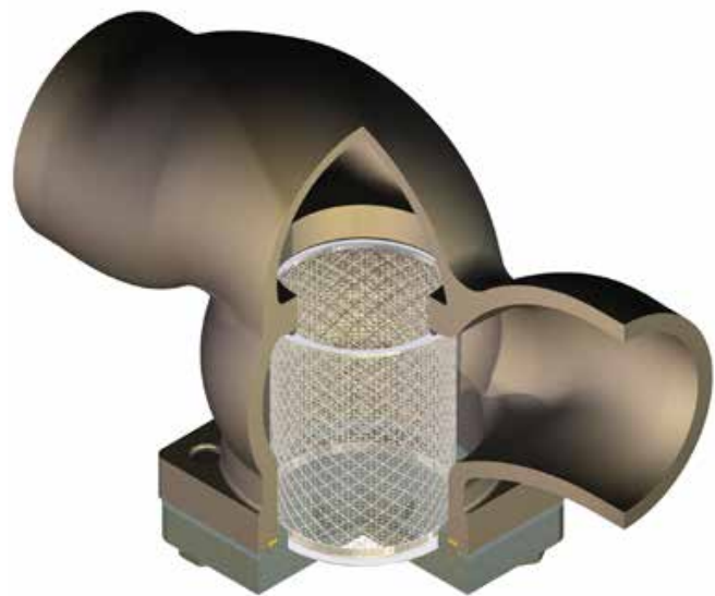
T5VA.F-SS, DN100
