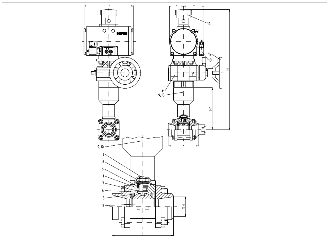
Dimensionen [mm] / Dimensions [mm]
