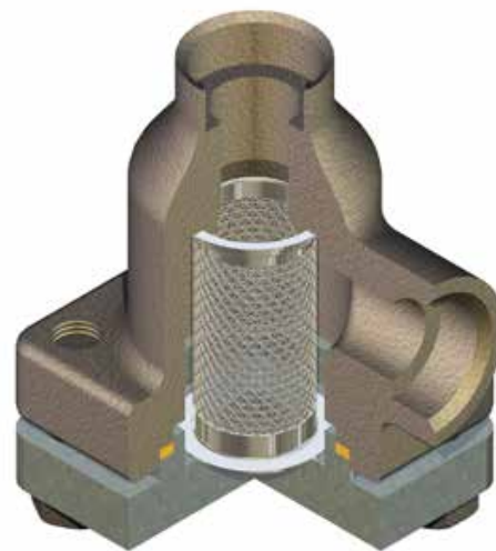
T61F-SS, DN25
