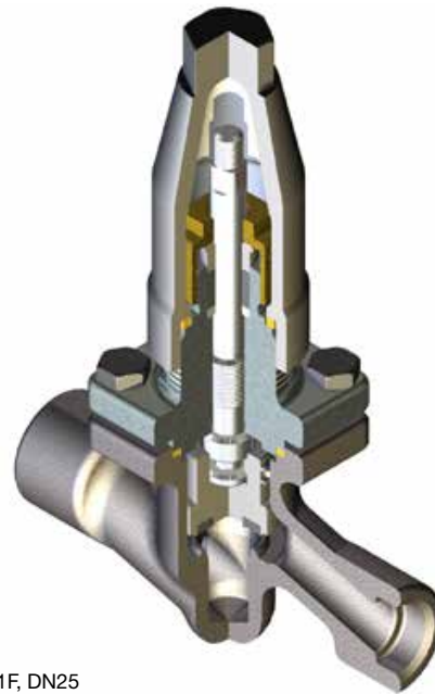
T51F, DN25
