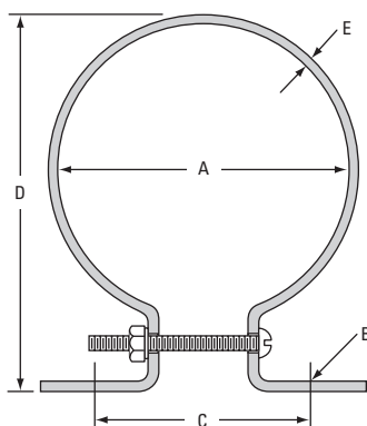
Mounting Bracket Dimensions
