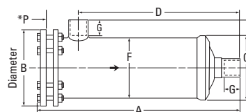
REPLACEABLE CORE TYPE
