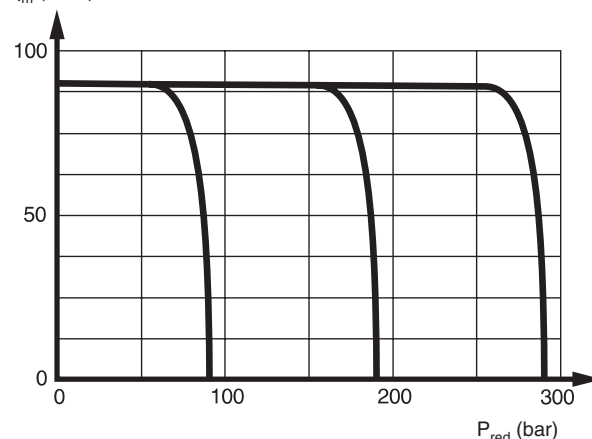
q_m (l/min) Feed reduction characteristics
