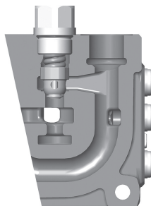
PA1 – Direct acting pressure relief valve.
