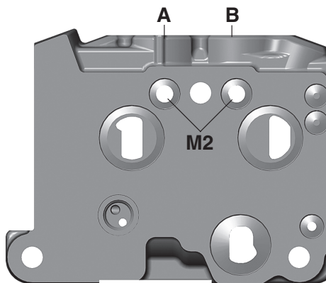
Worksection with internal connection of workports, M2.
