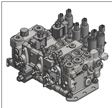
L90LS with work sections and function manifolds.
