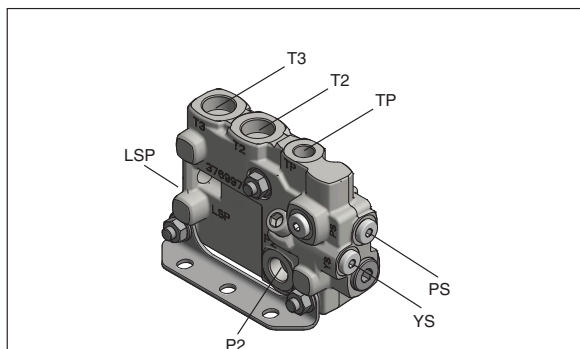
End section [P30] US
