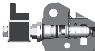
BEN – Electrically controlled pump-unloading function.
