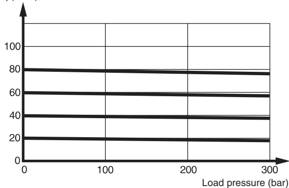
Load-independent flow with pressure compensator.
