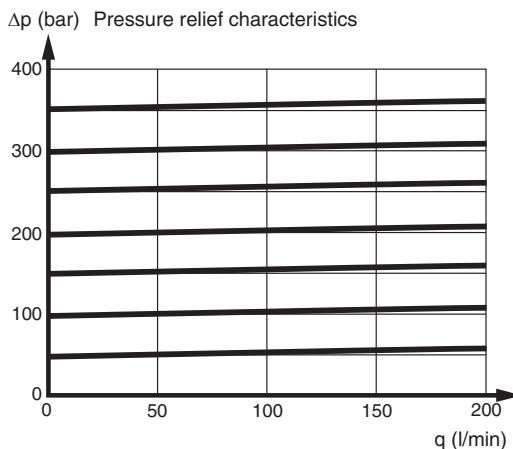
PS - Pilot-operated pressure relief valve
