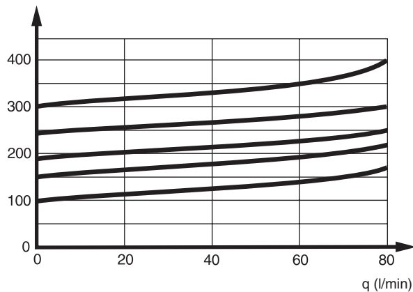
\Delta p (bar) Anti-cavitation characteristics
