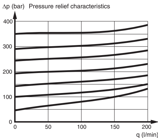
PA1 - Direct acting pressure relief valve.
