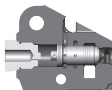
BX – Connection of signal pressure.
