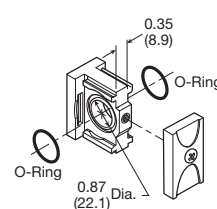
Body Connector
