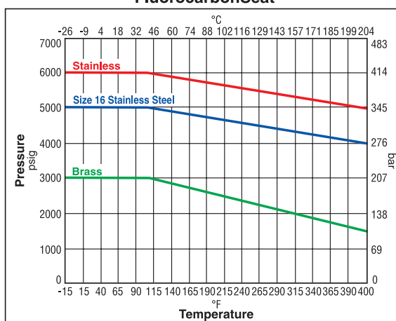
Fluorocarbon Seat
