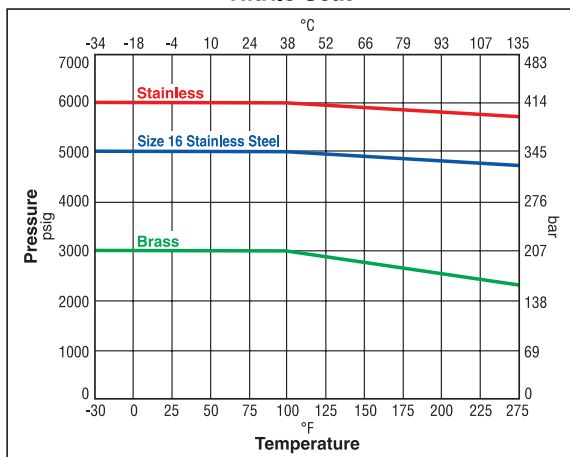
Nitrile Seat
