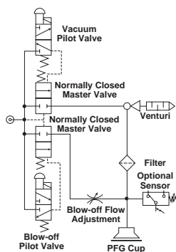
MC22, Normally Closed Vacuum Valve
