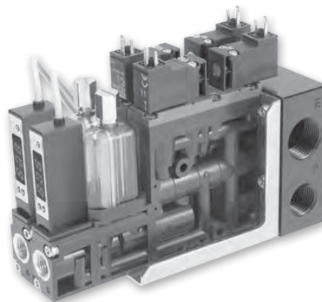
Add-A-Fold assembly (Silencer included)
