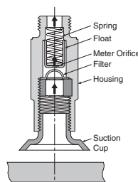
Figure 1 (Closed, Metered Flow)
