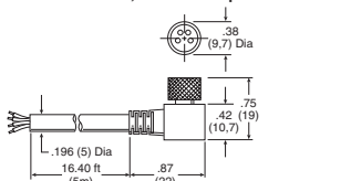
CB-M8-4P-5M-90, Female to Open Lead
