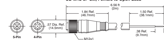
Female Interface 5-Pin, M12
