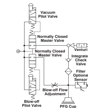
MC22, Normally Closed Vacuum Valve with Integrated Check Valve
