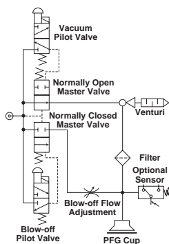
MC22, Normally Open Vacuum Valve
