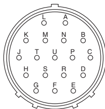
Face View - Male 18-Pin Connector
