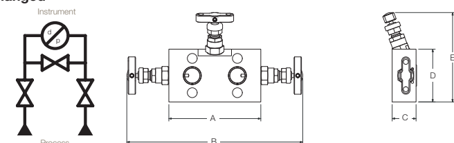
Example shown: 3-valve manifold with PTFree connect™ connection.
