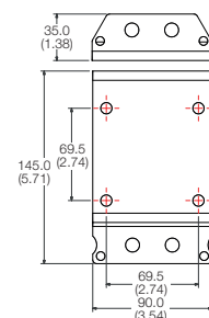
Image shown: Part No.: HDS3MBK
