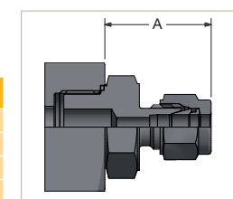
PTFree connect™ male connector (Code PFC)
