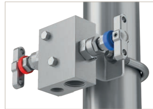
Image shown: Part No.: HLS2VBK
