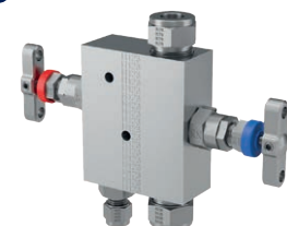
Example shown: 2-valve manifold with integral A-LOK® connections.
