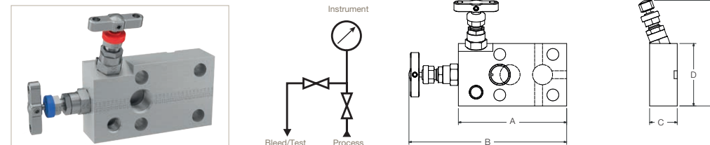
HD*2MCP - Female threaded - NPT x Flanged
