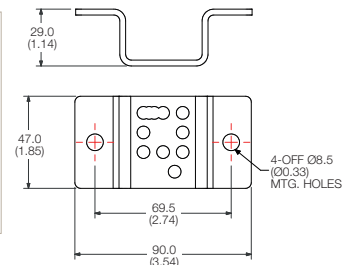
Image shown: Part No.: BKT1SSB1
