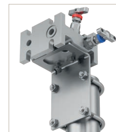
Image shown: Part No.: HEHS2BK
