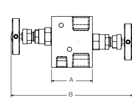
Example shown: 2-valve manifold with integral A-LOK® connections.
