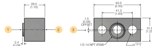
Example shown with traditional 1/2" NPT Fem. connection. Example shown with integral A-LOK® connection. Example shown with inverted integral A-LOK® connection.
