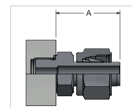
PTFree connect™ tube stub (Code PF)
