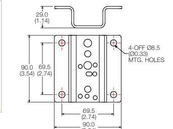
Image shown: Part No.: BKT2SSB2
