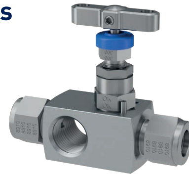
Example shown: Multi-port gauge valve with integral A-LOK® connections.
