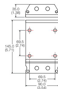
Image shown: Part No.: HDS3MCPBK
