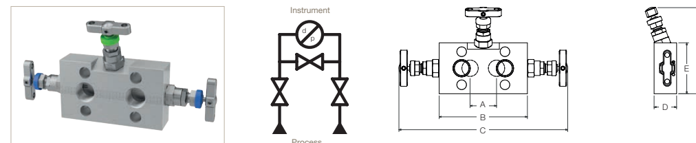
HD*3MCP - Female threaded - NPT x Flanged
