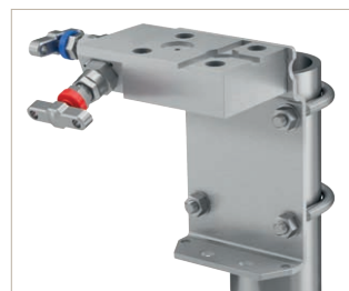
Image shown: Part No.: HDS2MCPBK
