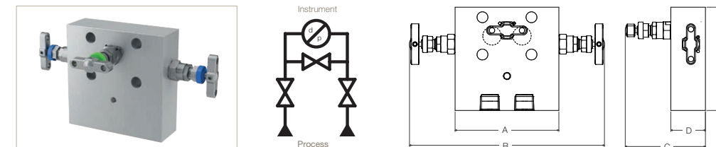
HD*3MCPEXT - Female threaded - NPT x Flanged
