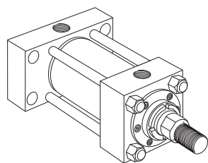
Style HH Rectangular Cap (NFPA Style ME6)
