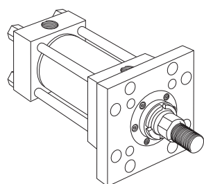
Style JB Head Square Flange (NFA Style MF5)
