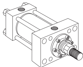
Style JJ Rectangular Head (NFPA Style ME5)
