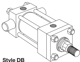
Style DB Cap Trunnion (NFFA Style MT2)
