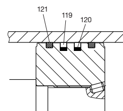
Hi-Load Piston
