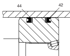
Lipseal Piston
