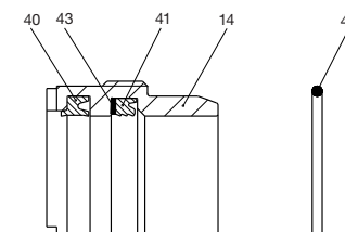
Gland Cartridge and Seals
