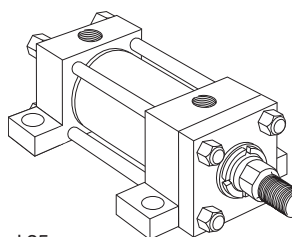
Styles C, F, G
