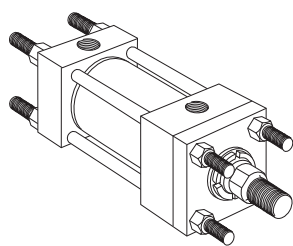
Style TD Tie Rods Extended Both Ends (NFPA Style MX1)
