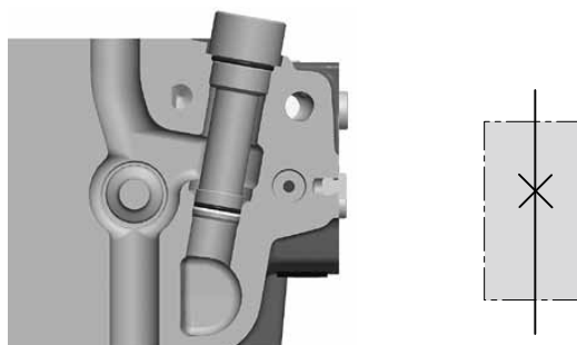
No port-relief or anti-cavitation valve fitted. Connection service port to tank gallery is blocked, type Y2.
