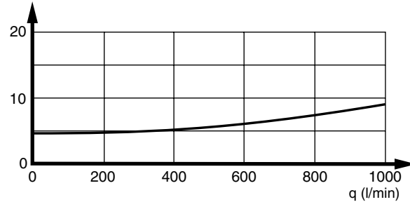
\Delta p (bar) Pressure drop over counter pressure valve
