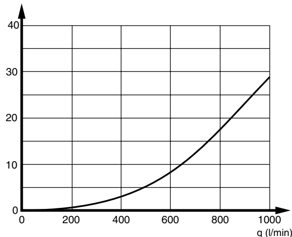
Pressure drop from service port A/B to tank connection T.
