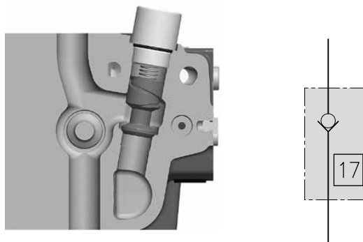
Anti-cavitation valve type N2.
