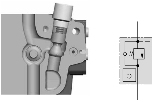
Port relief valve type PA.
