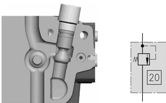
Port relief valve type PAY.
