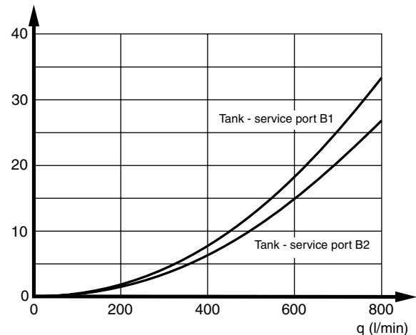
\Delta p (bar) Anti-cavitation characteristics
