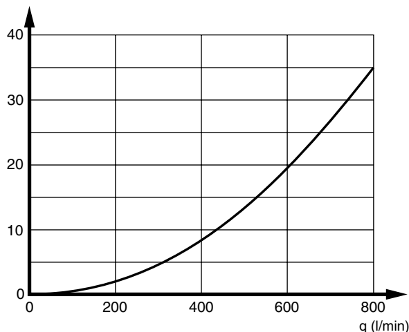
Pressure drop from pump connection P1/P2 to service port A/B.
