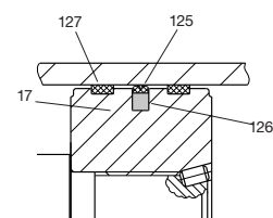
Standard Piston
