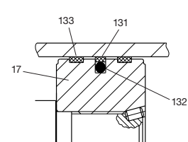
Low Friction Piston
