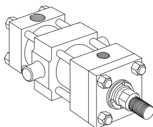
Style DD Intermediate Fixed Trunnion
