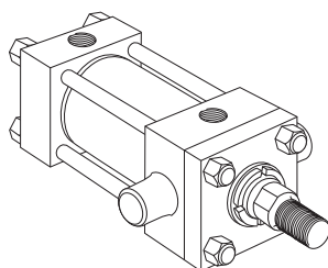
Style D Head Trunnion
