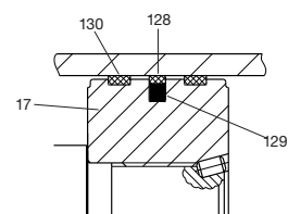
LoadMaster Piston
