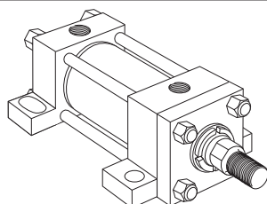
Style C Side Lugs
