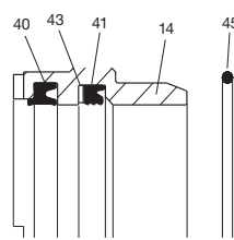
Gland Cartridge and Seals
