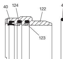
Low Friction Gland and Seals
