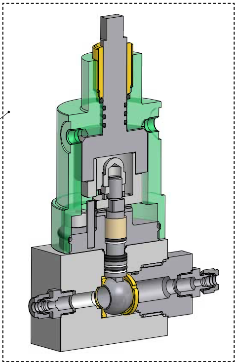
Ball valve ISO 15848-1 Prototype testing assembly
