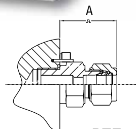
PTFree male connectors (Code FRCM)
