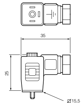
Connector with large headed screw
