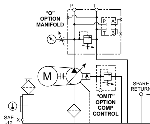
V-PAK BASIC UNIT
