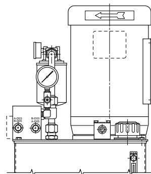
"O" & "S5" OPTION MANIFOLD (P & T BLOCK & D05 SINGLE STATION) SHOWN WITH OPTION "O" RETURN FILTER
