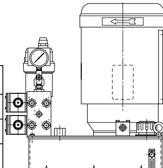
"M5" OPTION MANIFOLD (MULTI-STATION D05 MANIFOLD) SHOWN WITH OPTION "N" RETURN FILTER
