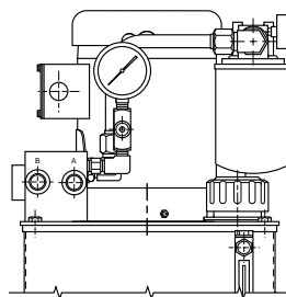
"O" & "S3" OPTION MANIFOLD (P & T BLOCK & D03 SINGLE STATION) SHOWN WITH OPTION "O" RETURN FILTER
