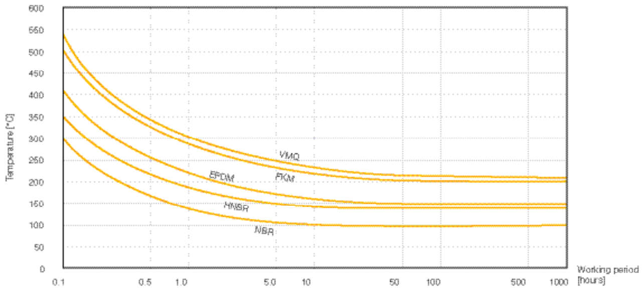
Fig. 7.1 High-temperature limits for various elastomeric materials
