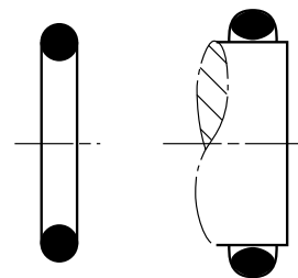
Fig. 8.12 left: unstretched O-ring, right: stretched O-ring
