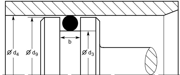
Fig. 3.9 Piston seal – radial compression
