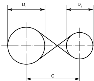
Fig. 2.20 Crossed design
