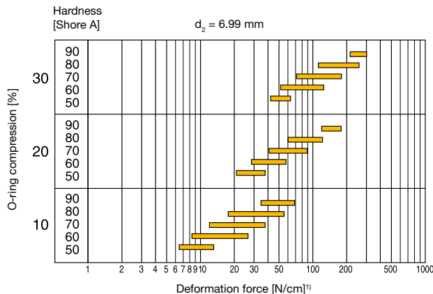
1) Length of O-ring circumference (cm) Fig. 8.30
