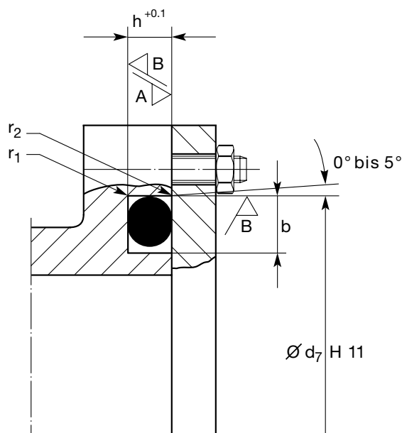
Fig. 2.8 Pressure from inside
