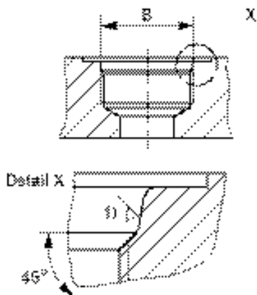
Dimensions for the conical counterbore are taken from the standard. Fig. 4.1 Threaded connector with conical counterbore
