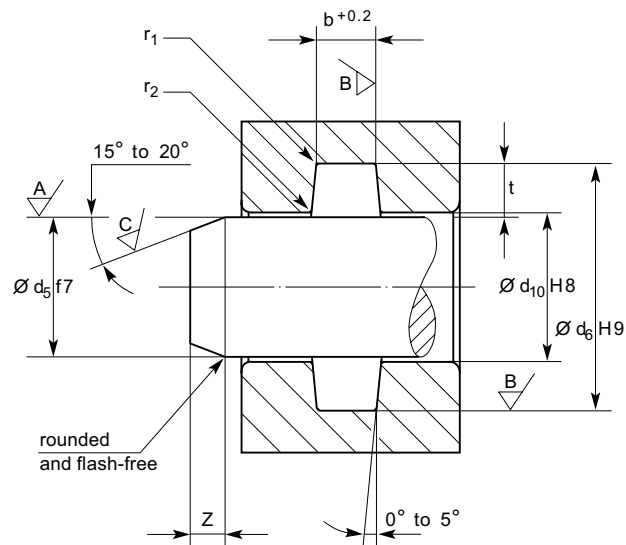
Fig. 2.6 Gland in outside element
