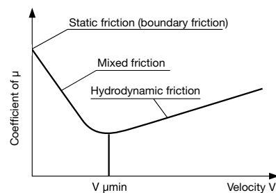
Fig. 8.18 Stribeck curve
