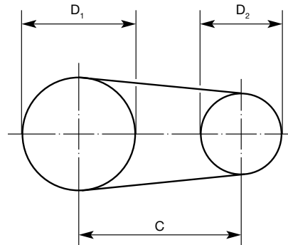
Fig. 2.19 Open design
