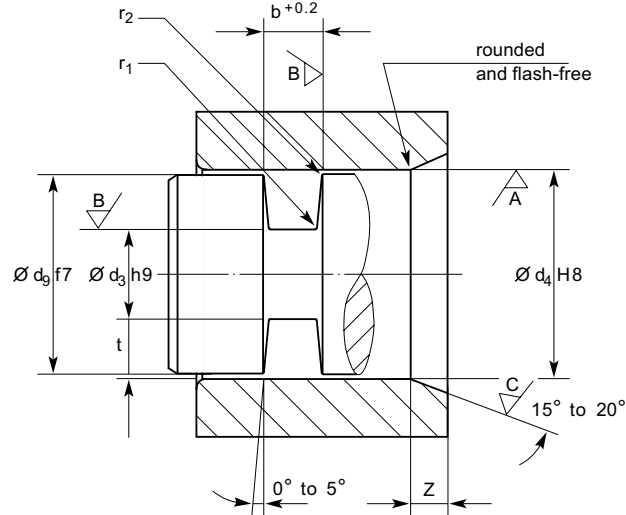
Fig. 2.5 Gland in inside element
