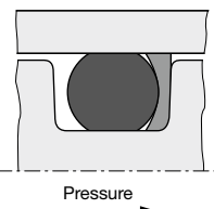
Fig. 10.4 The back-up ring on the non-pressurised side prevents gap extrusion.
