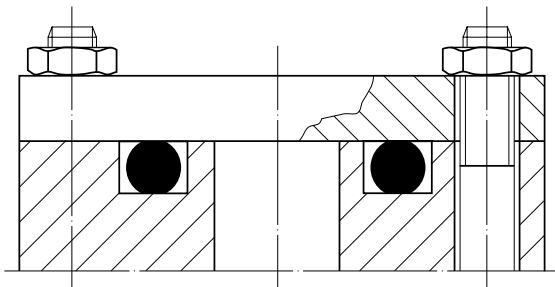
Fig. 2.3 Face seal: O-ring with axial compression
