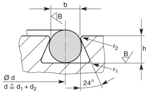
d = gland mean diameter The gland width is measured before deburring the edges. Radius r_2 is selected so that the O-ring is not damaged during assembly and cannot be trapped in the gap under high pressure. Fig. 2.11 Dovetail gland
