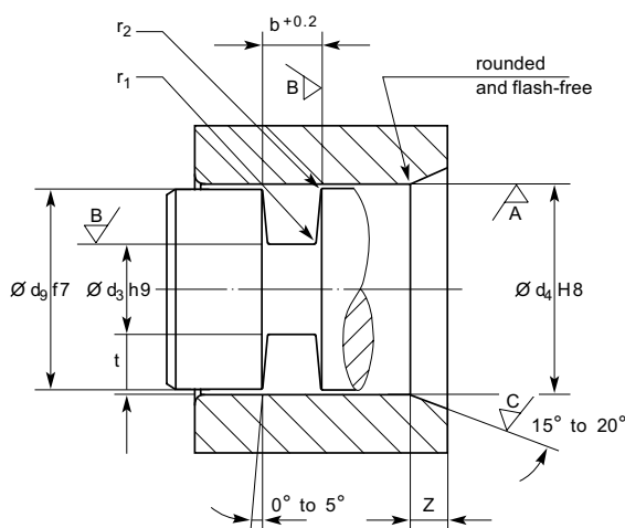
Fig. 2.15 Piston seal – hydraulic and pneumatic
