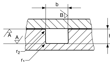
Fig. 7.6 Dimensions of vacuum gland, static application
