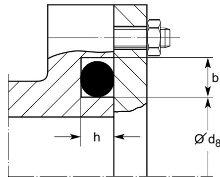
Fig. 3.4 Flange seal – axial compression
