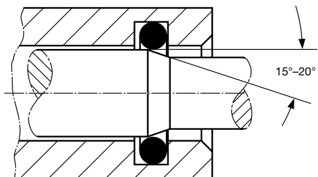
Fig. 2.23 Assembly example of rod
