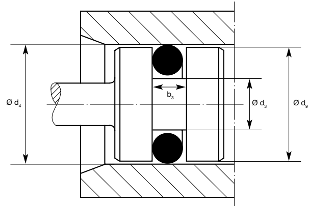
Fig. 3.15 Floating design – no compression
