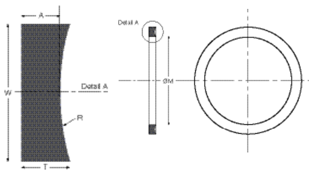
Fig. 4.11 Parbak® back-up ring
