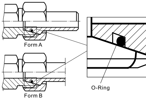
Fig. 4.4 Assembly
