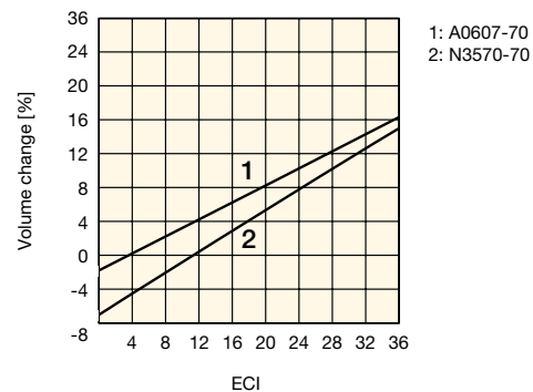
Fig. 8.7 Swelling characteristics of Parker compounds
