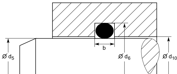
Fig. 3.2 Rod seal – radial compression
