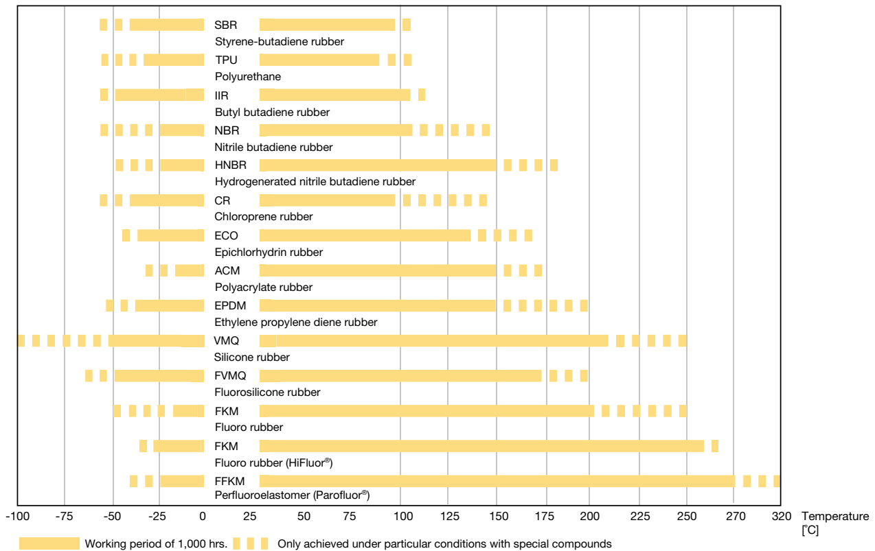
Fig. 7.1 High-temperature limits for various elastomeric materials
