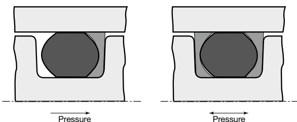
Fig. 4.9 Function of an O-ring-Parbak® combination
