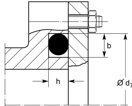
Fig. 3.3 Flange seal – axial compression
