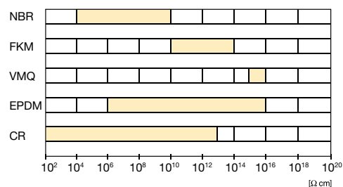
Fig. 8.9 Specific electrical resistance (according to DIN 53596)
