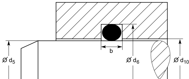
Fig. 3.14 Rod seal – radial compression
