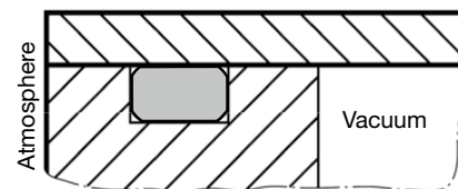
Fig. 7.5 Vacuum O-ring gland
