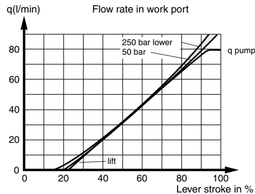
In the P70CP equipped with FPC, PC, ECS and ECH closed spool-actuators, the spools are pressure compensated, with the result that the load's influence on speed is negligible.
