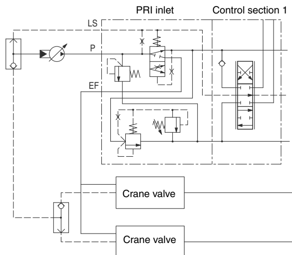
Inlet PRI in a system with variable pump
