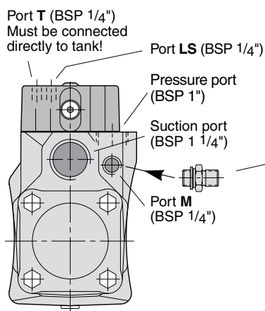
VP1-045/-060/-075 end view (showing ports).
