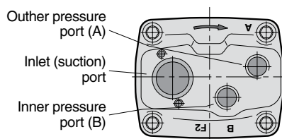
End cap for left hand rotating pump
