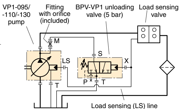
BPV-VP1 installation schematic with VP1-095/-110/-130 pump.
