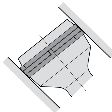
F1 piston with laminated piston ring.
