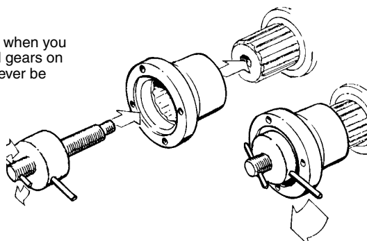
Fig. 7 Mounting tool.
