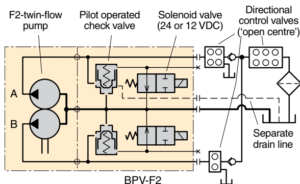
Bypass valve circuit schematic (example).
