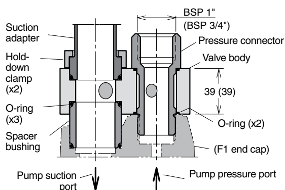
Bypass valve schematic.
