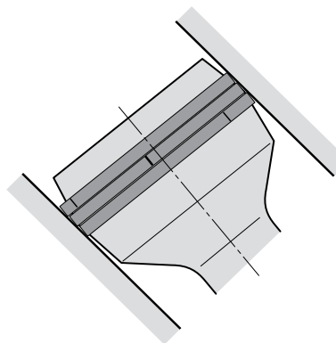
F3 piston with laminated piston ring.
