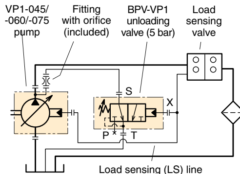
BVP-VP1 installation schematic with VP1-045/-060/-075 pump.
