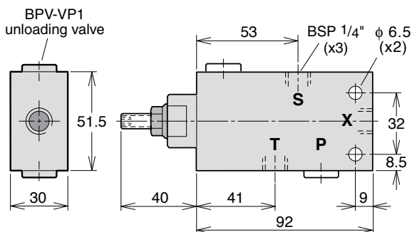
BPV-VP1 unloading valve.
