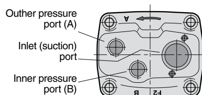
End cap for right hand rotating pump
