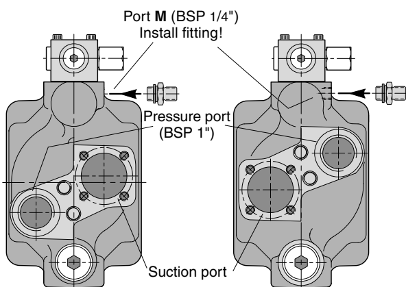
Left hand rotating pump Right hand rotating pump VP1-095/-110/-130 main ports (with fitting installation).
