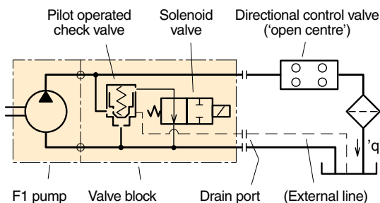
Bypass valve schematic.
