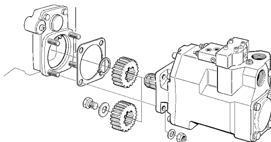
Fig. 6. VP1-to-PTO installation.
