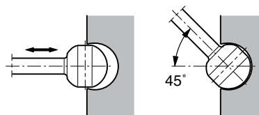
F3 piston-to-shaft locking.
