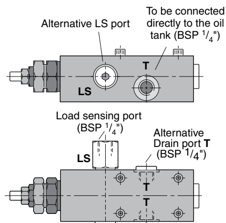
LS control ports.
