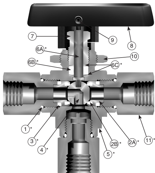
Model Shown: 4F-B6XJ-SSP
