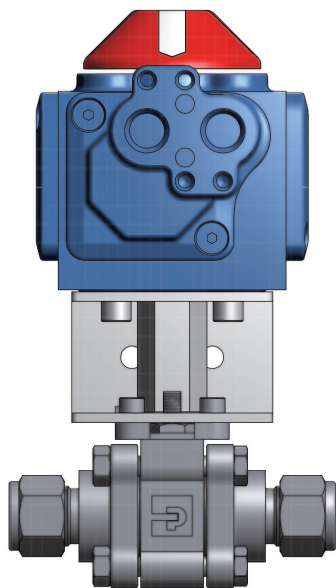
Pneumatic Actuated Model Shown: 8Z-SWB8L-RT-V-SS-51AD
