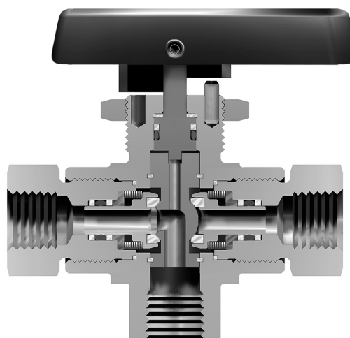
Three-Way HB4X Design
