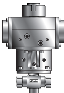
Spring Return (61AC & AO) Pneumatic Actuator
