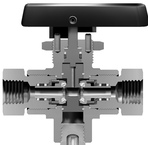
Two-Way HB4L Design
