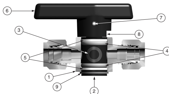
Model Shown: 4A-PR4-VT-SS
