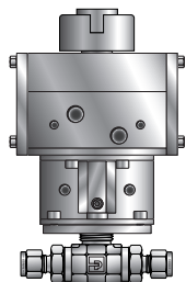
Double Acting (61AD) Pneumatic Actuator
