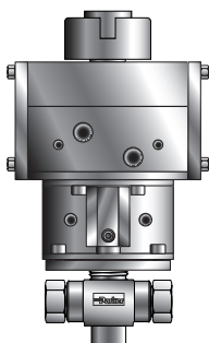
Double Acting (61AD) Pneumatic Actuator
