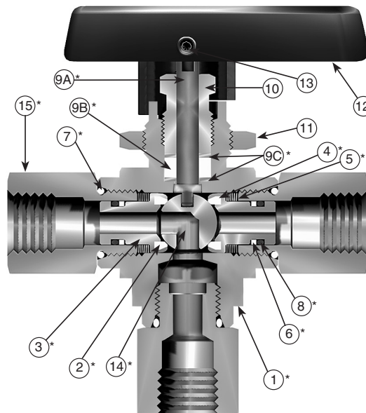
Model Shown: 4F-B6XS2-SSP
