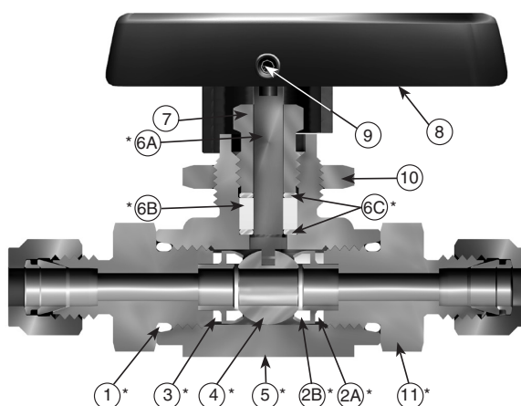
Model Shown: 6A-B6LJ-SSP
