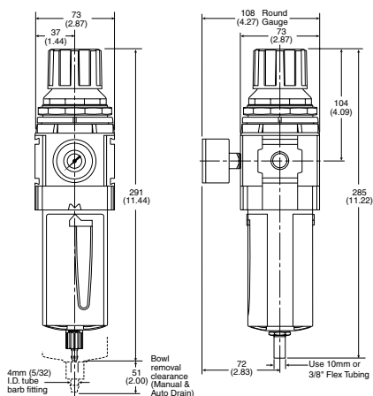
Automatic Drain
