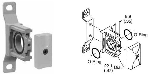
T-Bracket w/ Body Connector P32KA00MT
