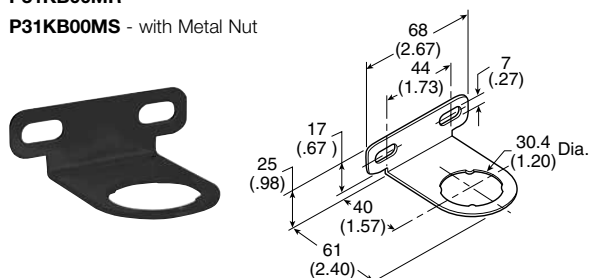
Angle Bracket (Fits to regulator and filter/regulator body)
