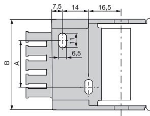
Standard carrier connection
