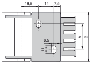
Standard fixed point connection (inelastic)
