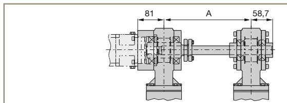
Center distance A between 150-350 mm
