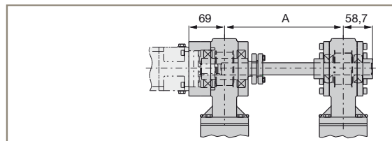
Center distance A between 150-350 mm
