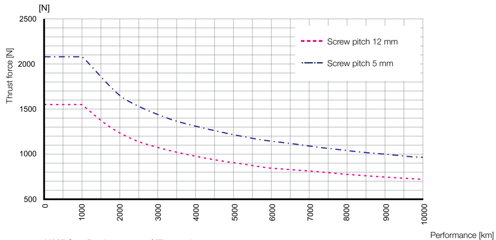
HMRS15 Performance / Thrust force
