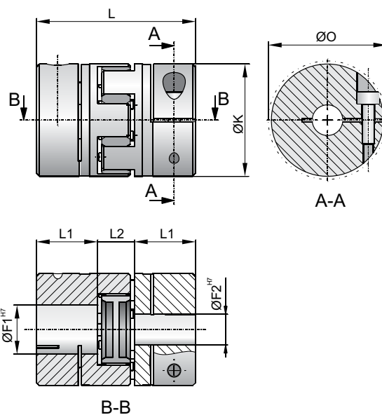
Dimension table - motor coupling HMRS [mm]
