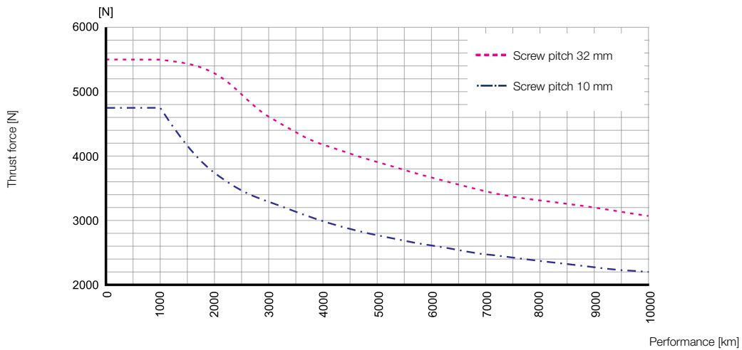
HMRS24 Performance / Thrust force
