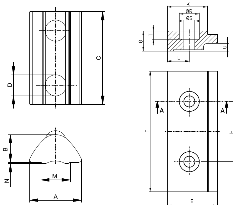
Dimension table - T-slot mounting HMR [mm]
