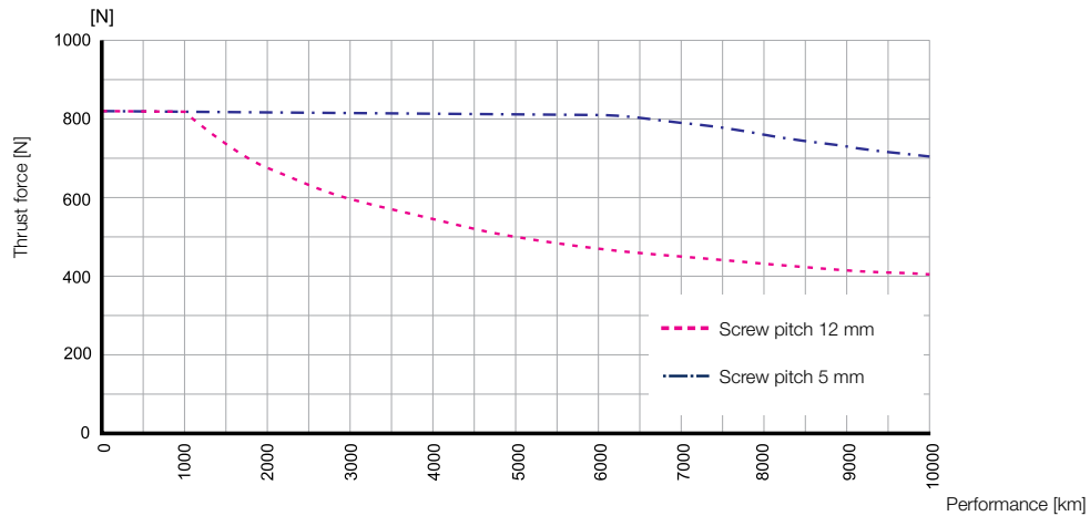
HMRS11 Performance / Thrust force
