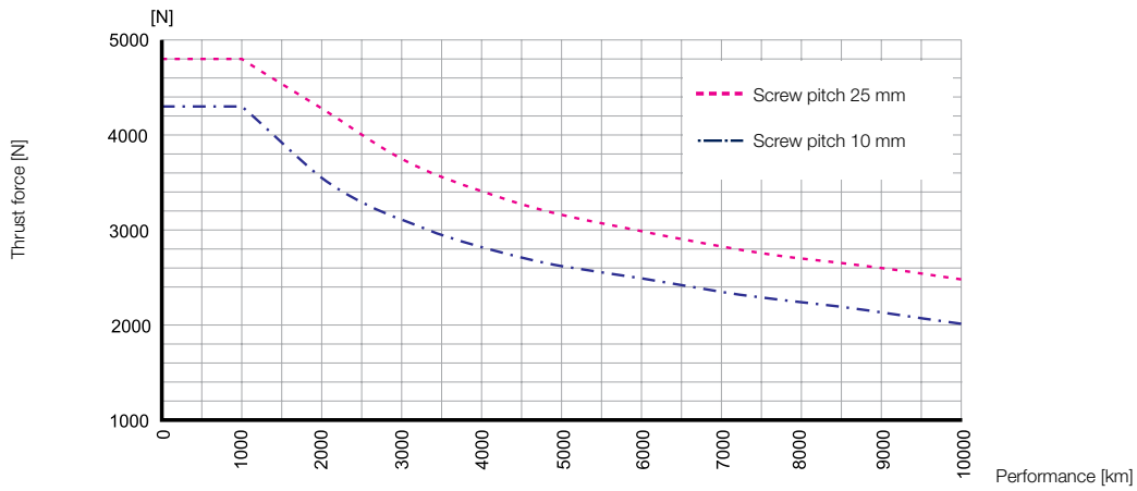
HMRS18 Performance / Thrust force
