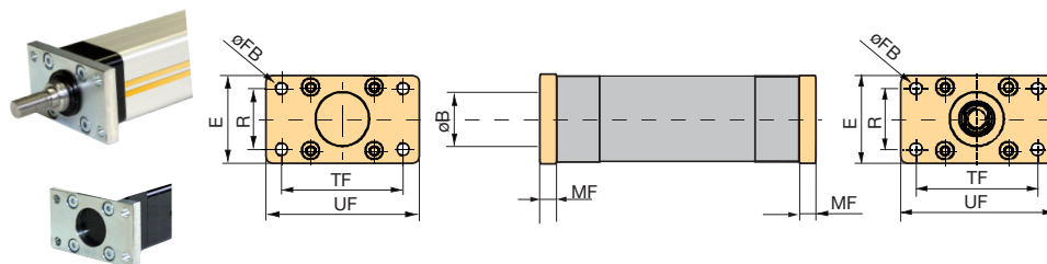
Front and rear plate dimensions
