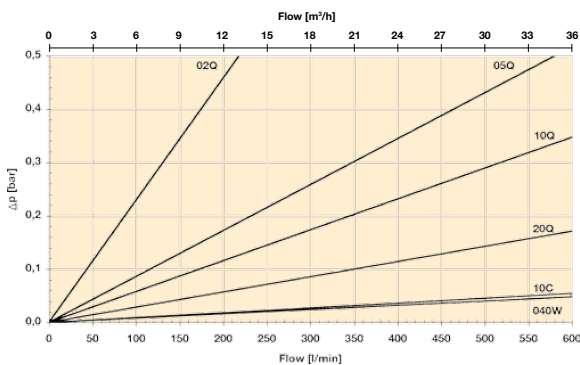
BGAH 3-500 elements (Length 12)
