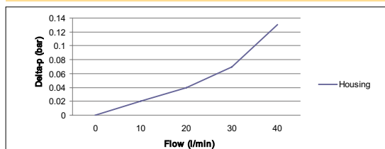
EPF Size 1 Empty housing
