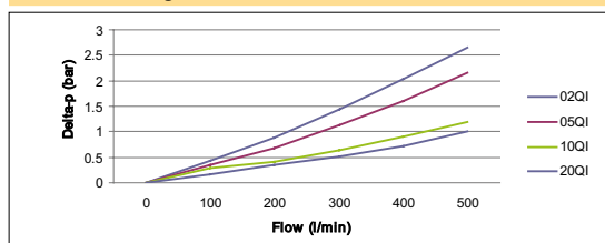
EPF Size 4 Length 1 Filter Elements
