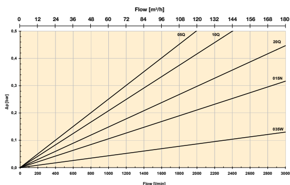
Length 3 element pack (3 pcs)/one side in use
