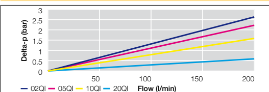
EMDPF Size 3 Length 1 Filter Elements
