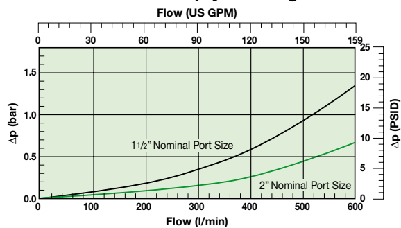
80CN Empty Housing
