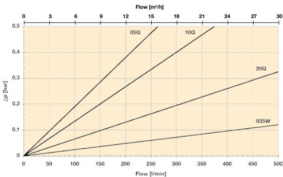
DF2089 elements/one side
