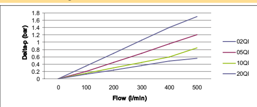
EPF Size 4 Length 2 Filter Elements
