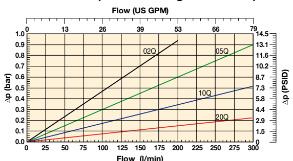
ETF175 (Element length code 4B)
