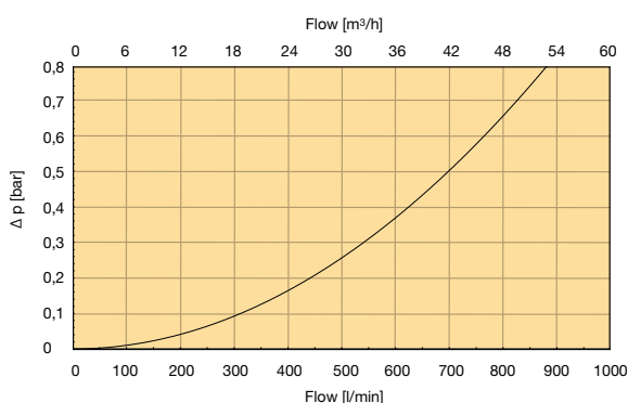
DF65 housing
