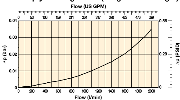
BGT800 (Element length code 14)
