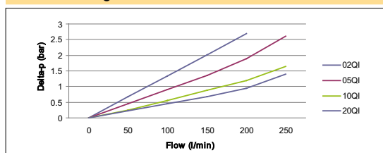
EPF Size 3 Length 1 Filter Elements
