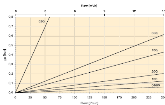
GA2-170 elements (Length 6)
