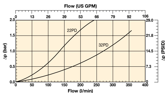
22PD/32PD Empty Housing
