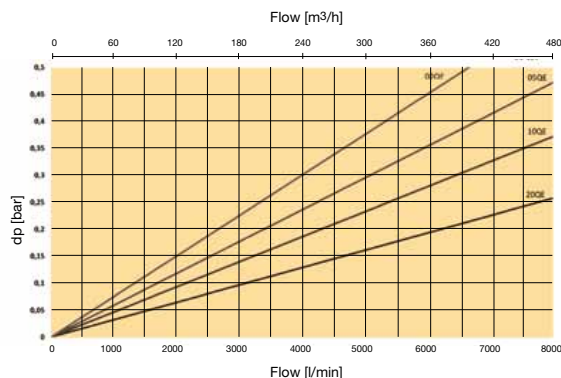
HFS/HFD43 (4 elements) QE element dp-curves
