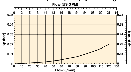
ATZ 1-120 (G1½) Empty Housing
