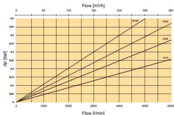
HFS/HFD83 (8 elements) QE element dp-curves
