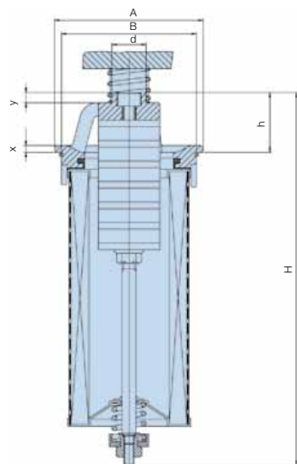
without diffuser
