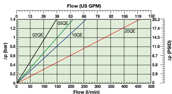
45M-1 Element with Ecoglass III
