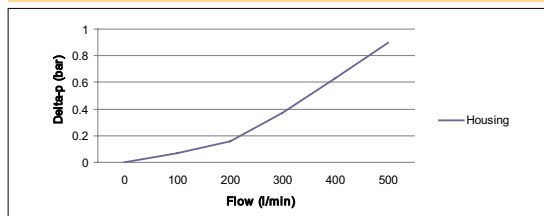
EPF Size 4 Empty Housing
