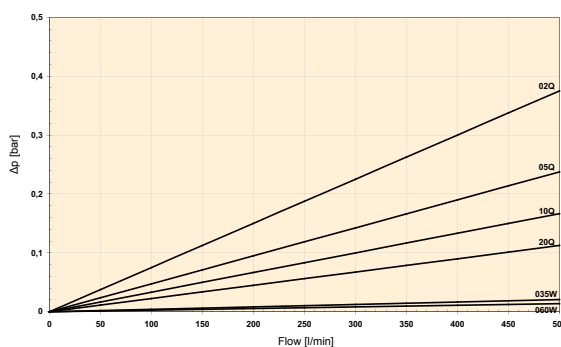
DF60 elements / both sides
