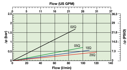
IN120 (Element length code 4)
