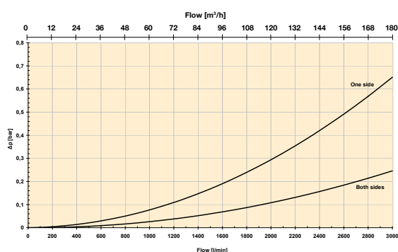
DFH2060 element pack (3 pcs)/one side in use
