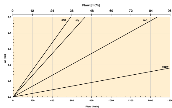
Length 3 element pack/one side
