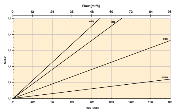
Length 3 element pack/one side
