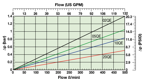
45M-3 Element with Ecoglass III
