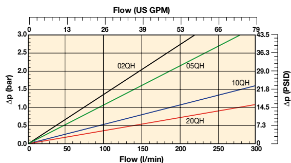
32PD-1 High Collapse Elements
