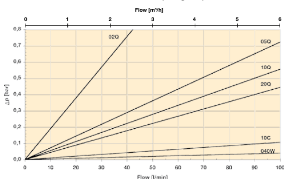
GA1-60 elements (Length 2)
