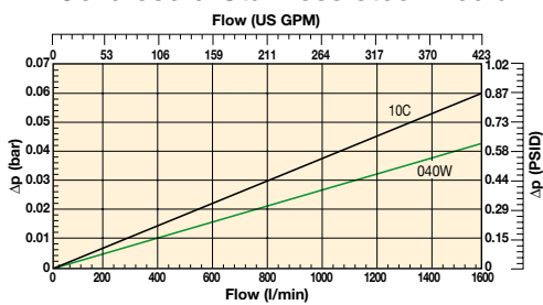
IN1500 (Element length code 16) Cellulose & Stainless steel media
