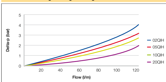
EAPF Size 1 Length 2 High Strength Filter Elements
