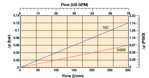
STF230 (Element length code 7) Cellulose & stainless steel media
