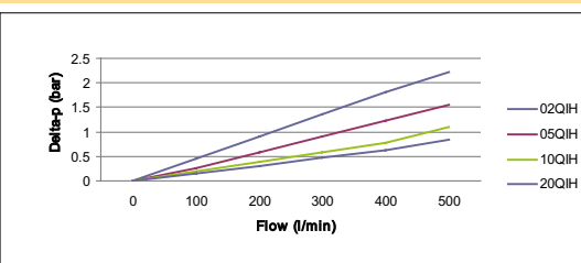
EPF Size 4 Length 2 High Strength Filter Elements
