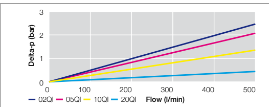
EMDPF Size 4 Length 1 Filter Elements
