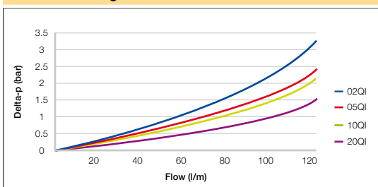
EAPF Size 1 Length 2 Filter Elements
