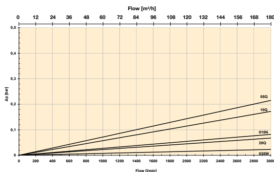
DFH2060 element pack (3 + 3 pcs)/both sides in use
