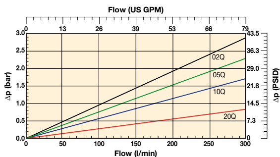
22PD-1 Elements
