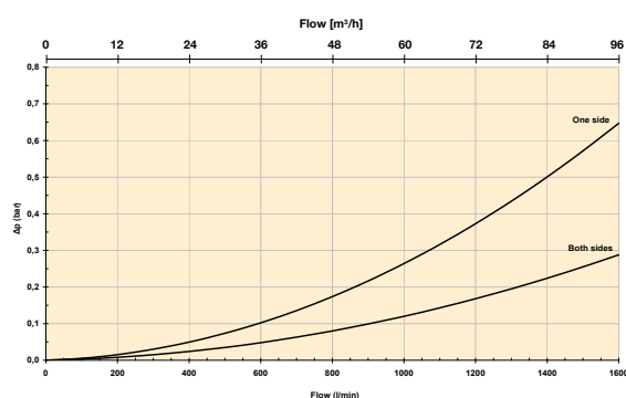
Length 2 element pack/one side
