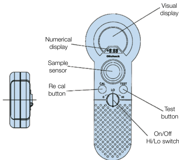
Function buttons
