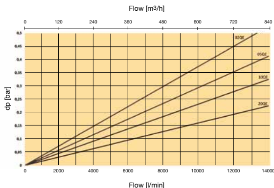
HFS/HFD83 (8 elements) QE element dp-curves
