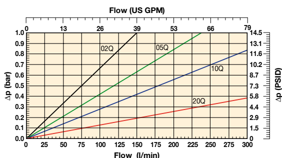
ETF175 (Element length code 4B)
