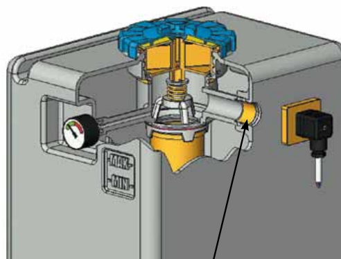
Customised integrated metal attachment "Tank also features integrated level measurement"
