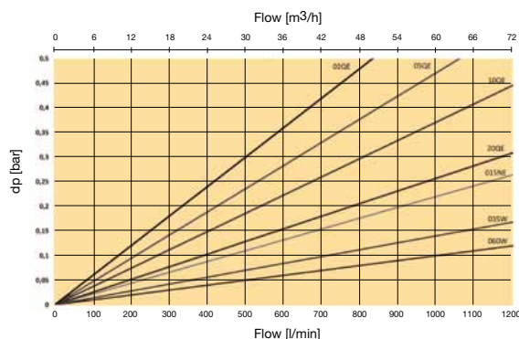
Single element: Length 2 Element dp-curves
