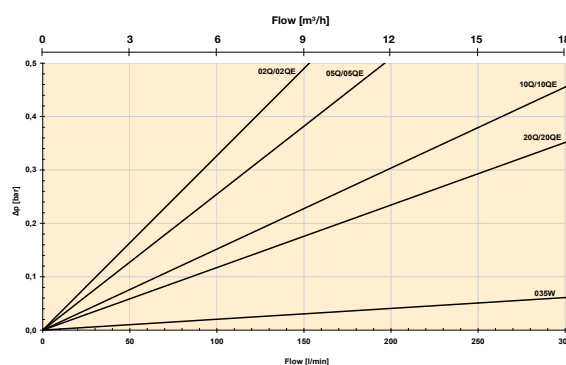
DF40 elements
