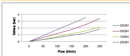
EPF Size 3 Length 1 High Strength Filter Elements
