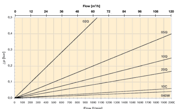
BGLS 4-2000 elements (Length 17)
