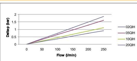
EPF Size 3 Length 2 High Strength Filter Elements
