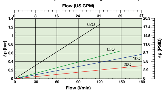
TTF120 (Element length code 4)
