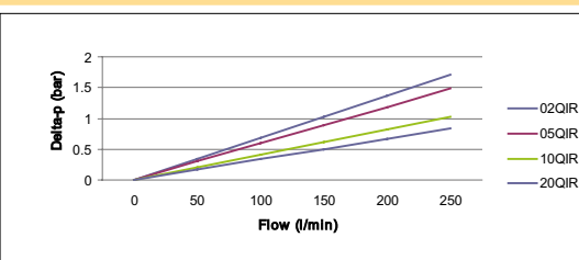
EPF Size 3 Length 2 Filter Elements with reverse flow valve
