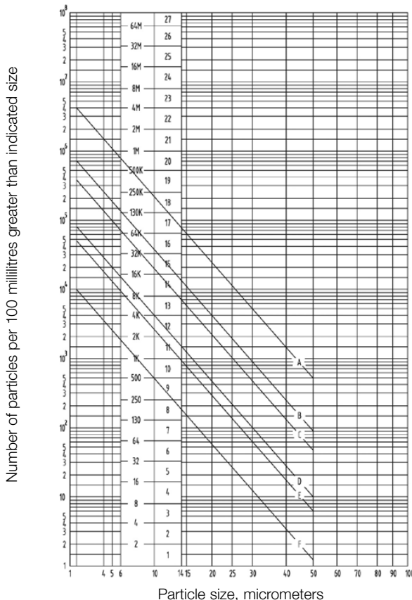
ISO 4406:1999 cleanliness classes
