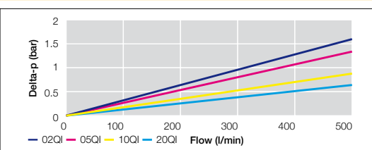
EMDPF Size 4 Length 2 Filter Elements
