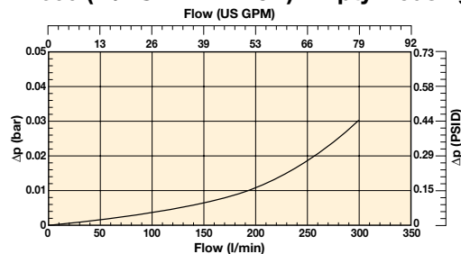
ATZ 300 (2½ SAE FLANGE) Empty Housing
