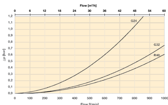
Length 2 elements
