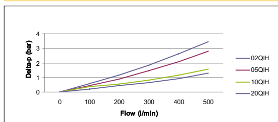
EPF Size 4 Length 1 High Strength Filter Elements
