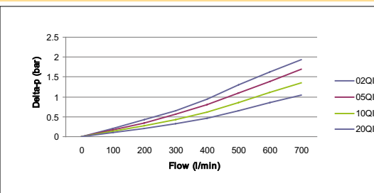
EPF Size 5 Length 1 Filter Elements
