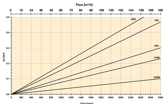
Length 3 element pack (3 + 3 pcs)/both sides in use
