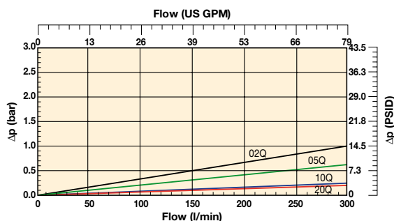
32PD-2 Elements
