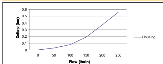
EPF Size 3 Empty Housing
