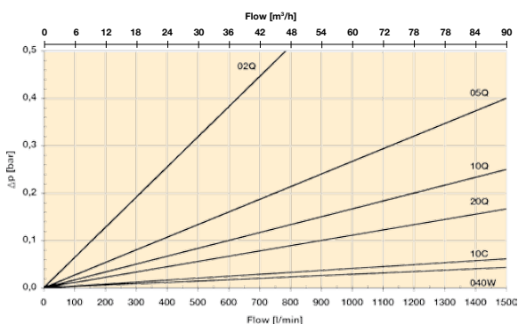
BGLS 4-1500 elements (Length 16)
