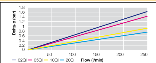
EMDPF Size 3 Length 2 Filter Elements
