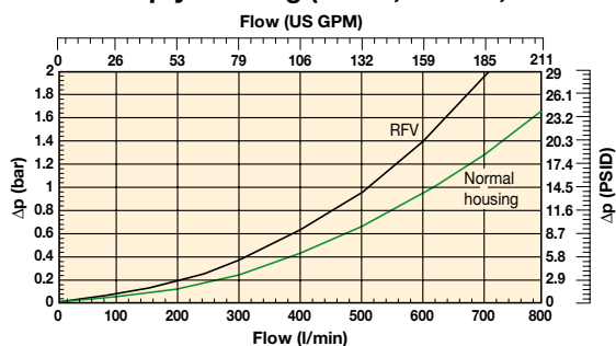
100P-1 Elements
