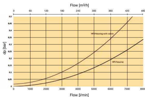
Single element: Length 2 Element dp-curves
