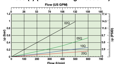
IN800 (Element length code 14)
