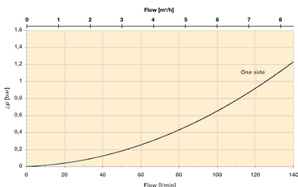
DF2145 housing
