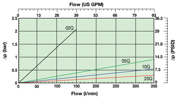
STF300 (Element length code 8)
