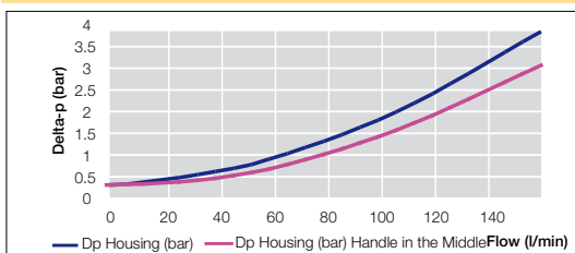
EMDPF Size 3 Length 2 Filter Elements
