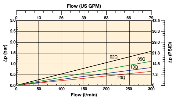
22PD-2 Elements
