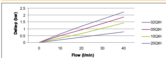
EPF Size 1 High Strength Filter Elements
