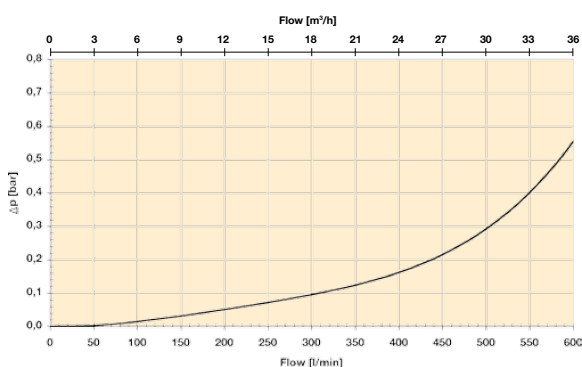
BGAH 3-400 elements (Length 11)
