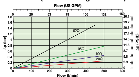
IN390 (3)(Element length code 11)
