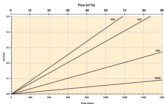
Length 3 element pack/both sides
