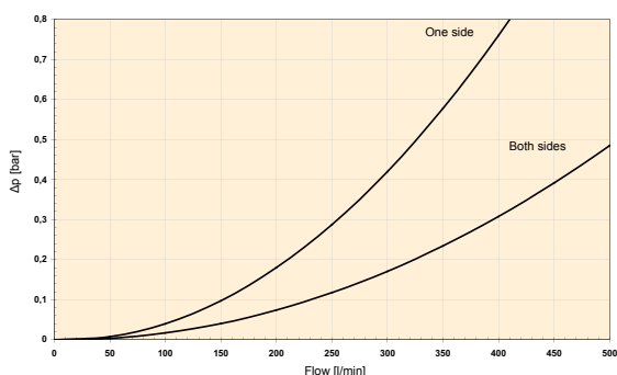
DF60 elements / one side
