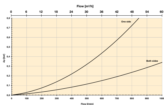
Length 2 element pack (2 pcs)/one side in use
