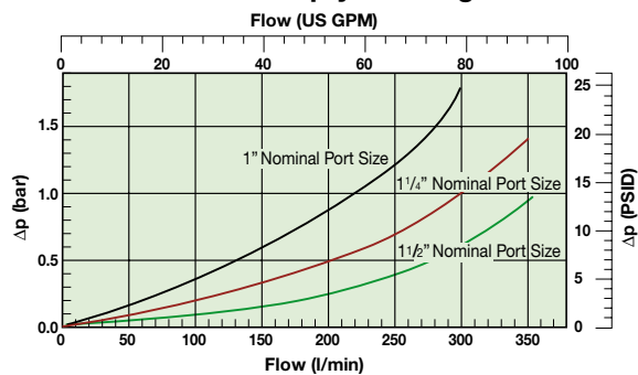
40CN Empty Housing
