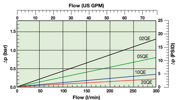
80CN-1 Elements
