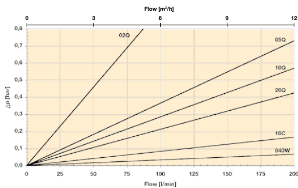
GA2-230 elements (Length 7)
