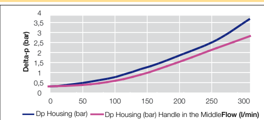
EMDPF Size 4 Empty Housing
