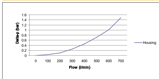
EPF Size 5 Empty Housing
