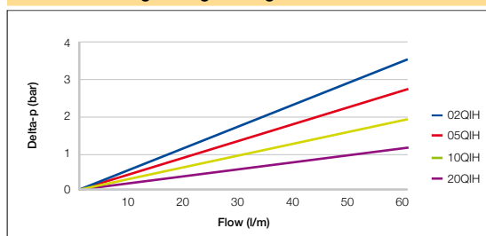
EAPF Size 1 Length 1 High Strength Filter Elements
