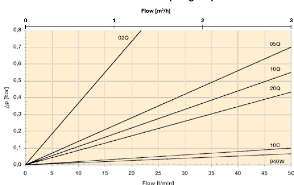
GA1-30 elements (Length 0)
