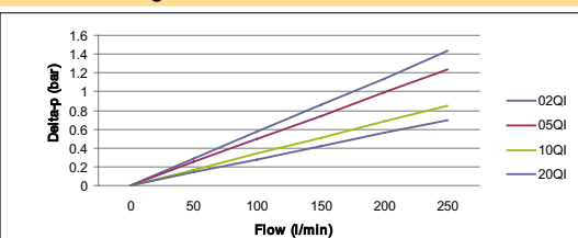
EPF Size 3 Length 2 Filter Elements
