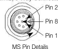
M12, 8 Way Connector
