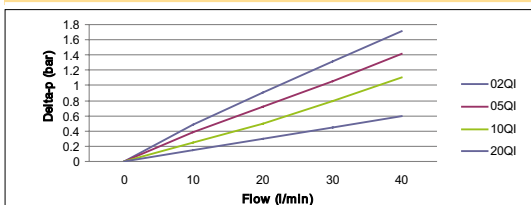
EPF Size 1 Filter Elements
