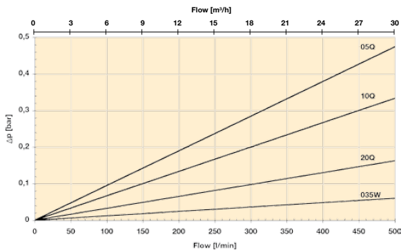
DF2089 elements/both sides
