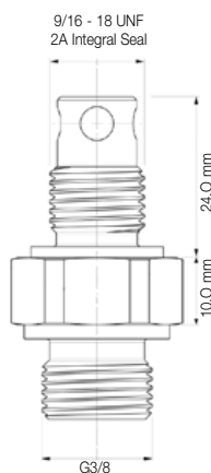
Thread Form Option 5
