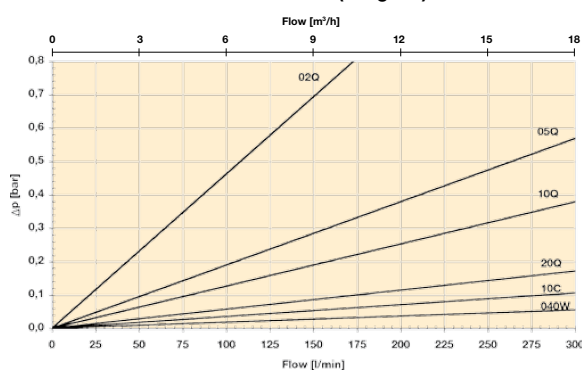
GA2-230 elements (Length 7)
