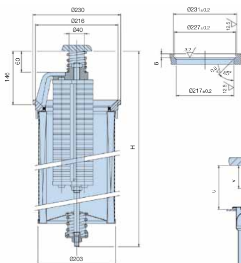
without diffuser
