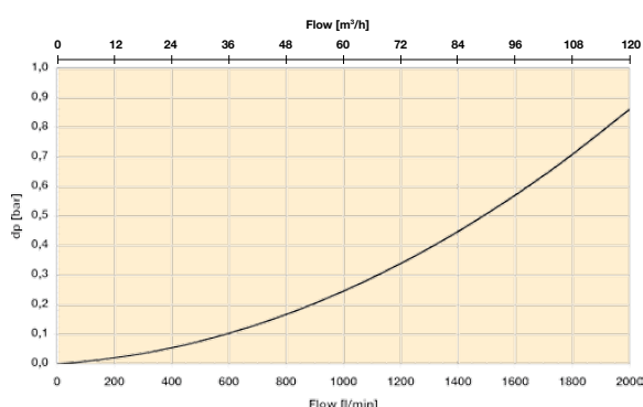
SF1040 DN80/PN16 housing
