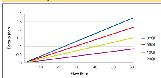
EAPF Size 1 Length Filter Elements
