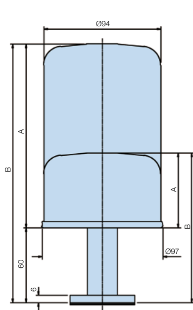
Standard spin-on air breather stem
