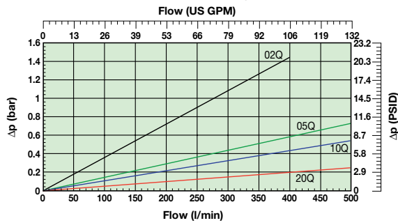
STF500 (Element length code 10)
