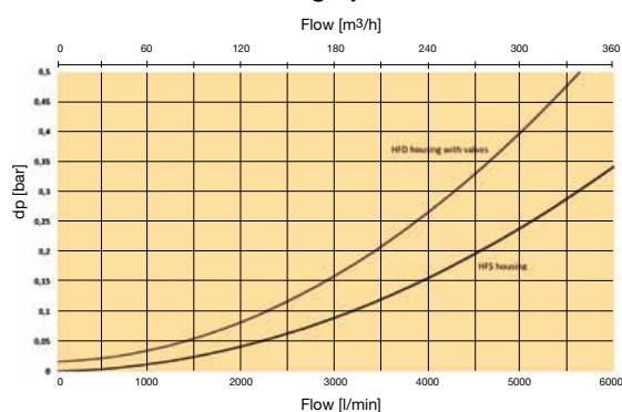
HFS/HFD83 DN350 (8 elements) Housing dp-curves
