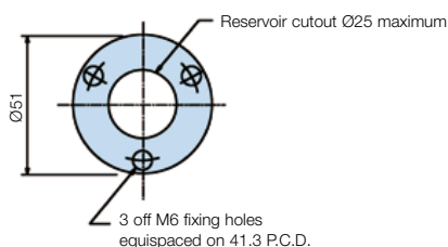
Standard spin-on air breather stem
