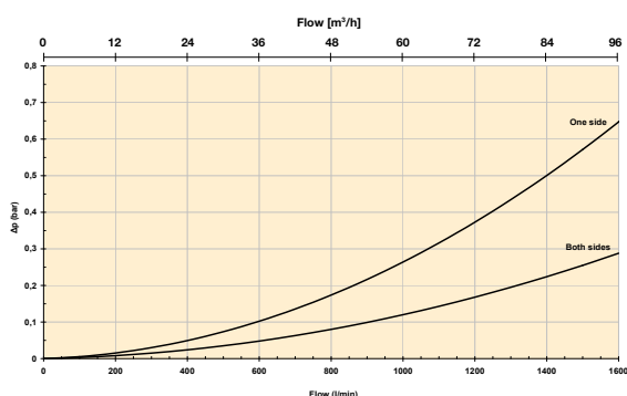
Length 1 elements/one side
