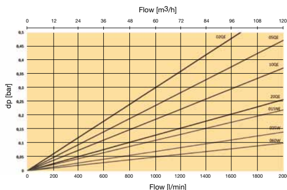
Single element: Length 3 Element dp-curves
