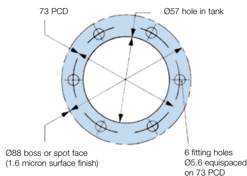
Mounting face for standard and large breather
