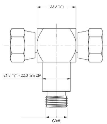
Thread Form Option 7
