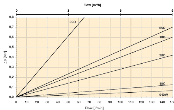
GA2-170 elements (Length 6)
