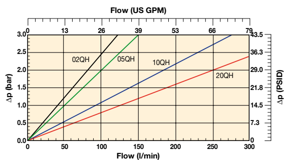
22PD-1 High Collapse Elements
