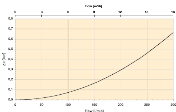
DF40 housing
