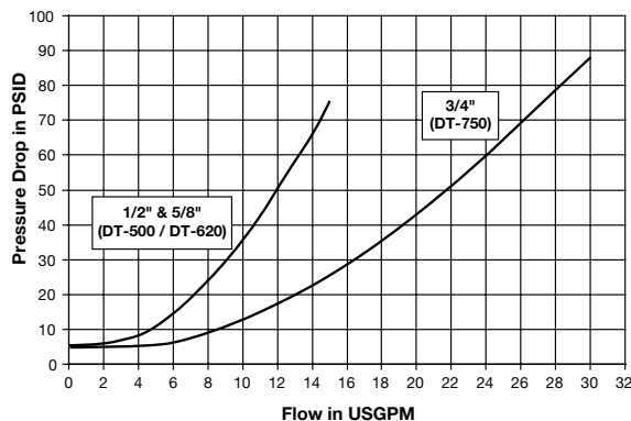
DT Series (1/2", 5/8" & 3/4") Test Fluid: Oil - 200 SUS
