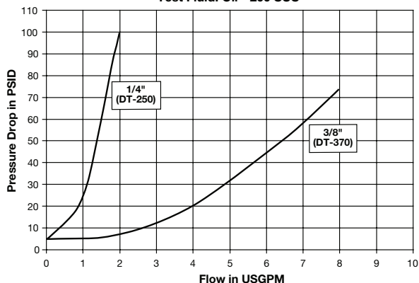
DT Series (1/4" & 3/8") Test Fluid: Oil - 200 SUS
