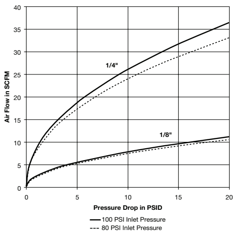
Performance HF Series (1/8" & 1/4" sizes)
