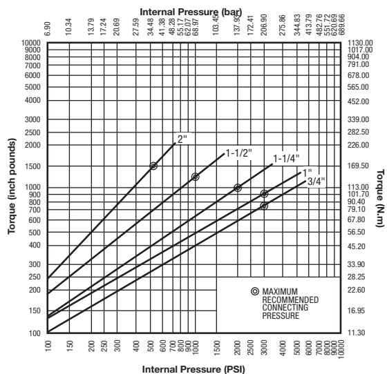
Torque Values for Connecting Under Pressure
