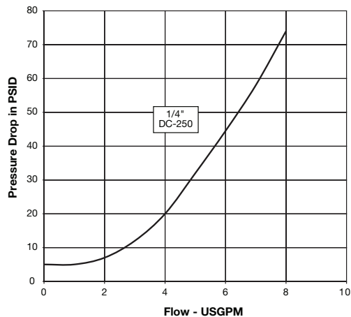
DC Series (1/4") Test Fluid: Oil - 200 SUS
