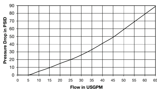
Inlet Port thru Tank Port @ 100°F (300 SUS)
