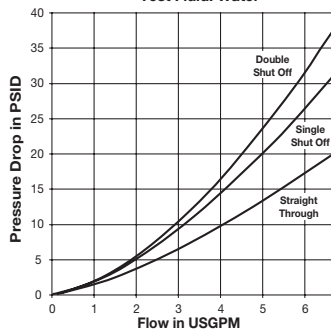
Spectrum Series (3/8") Test Fluid: Water
