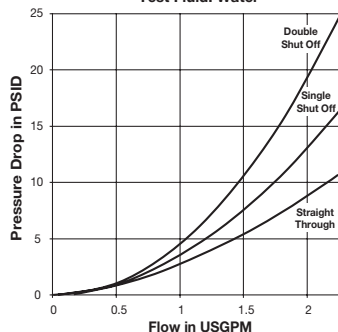
Spectrum Series (1/8") Test Fluid: Water
