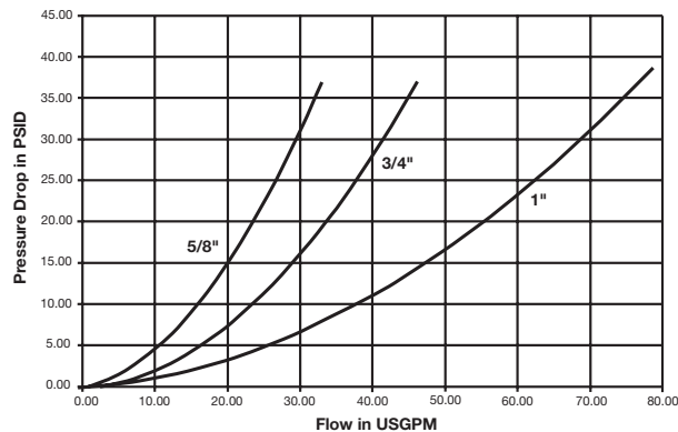
FEM Series (5/8", 3/4" & 1") Test Fluid: Oil - 150 SUS
