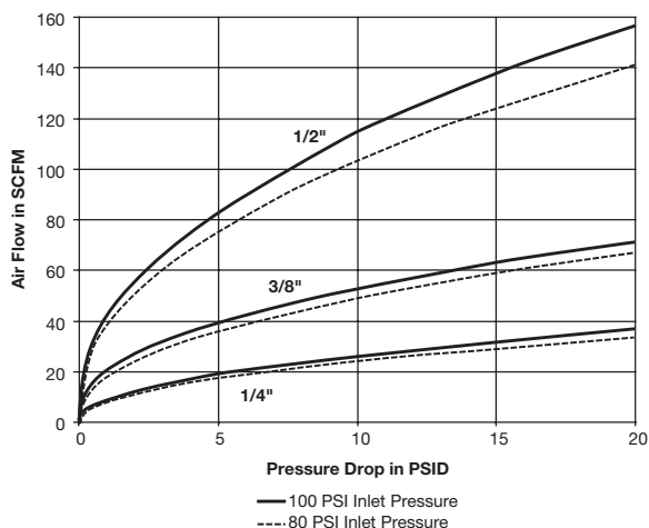
Performance 10 Series (1/4", 3/8", 1/2" sizes)
