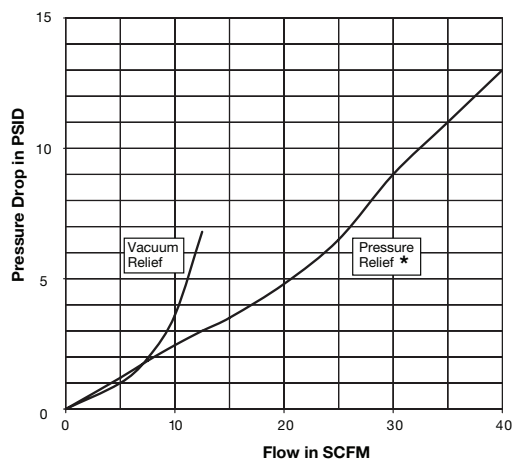
Flow Data PV Pressure-Vacuum Relief Valve
