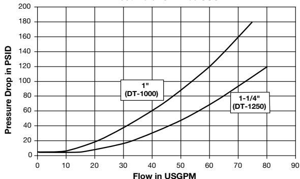
DT Series (1" & 1-1/4") Test Fluid: Oil - 200 SUS
