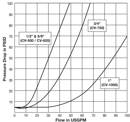
CV Series (1/2", 5/8", 3/4" & 1") Test Fluid: Oil - 200 SUS
