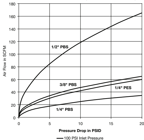
Tool-Mate Series Exhaust (1/4", 3/8" & 1/2" sizes)
