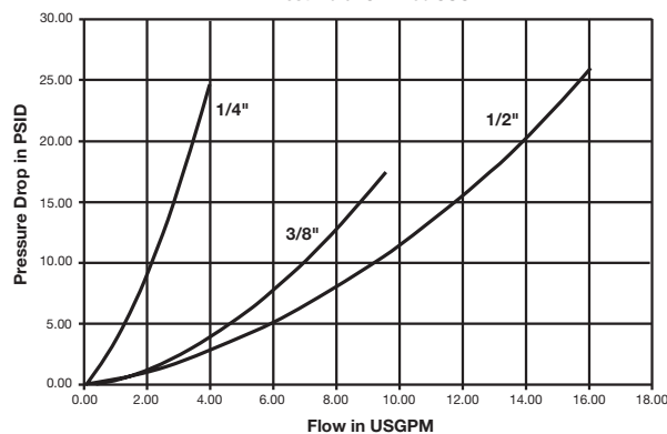
FEM Series (1/4", 3/8" & 1/2") Test Fluid: Oil - 150 SUS
