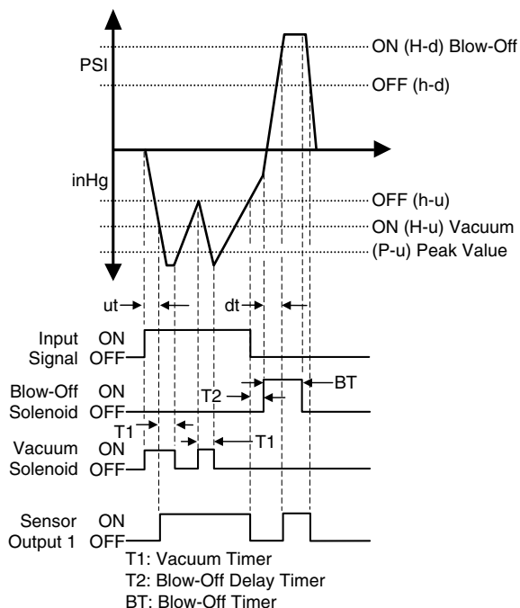
Mode: OP1 "Air Conservation / Timer"
