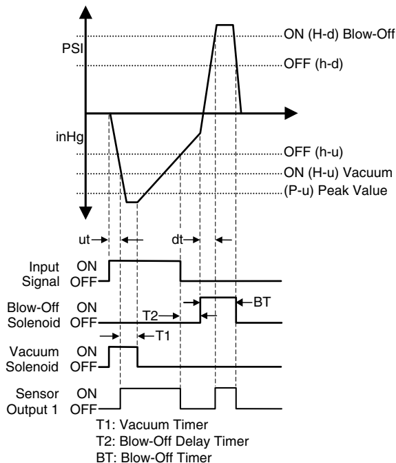
Mode: OP2 "Vacuum Timer Option"
