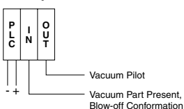
PLC System with 201 Sensor
