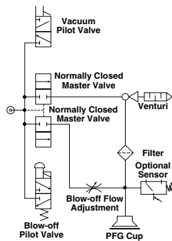
MC2, Normally Closed Vacuum Valve
