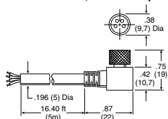
CB-M8-4P-5M-90, Female to Open Lead
