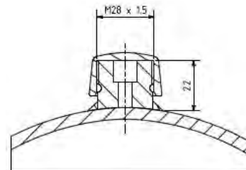
Gas Valve
