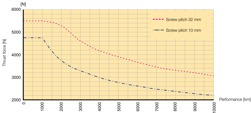
HMRS24 Performance / Thrust force
