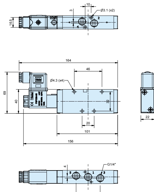
P2LBZ 5/2 Solenoid / Spring
