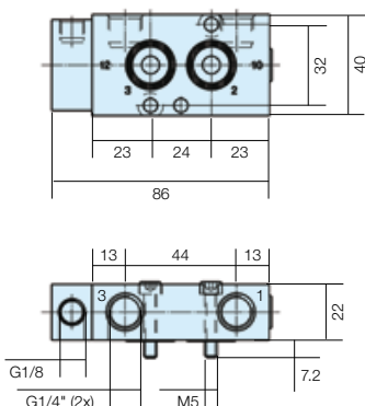
Dimensions Reference 7
