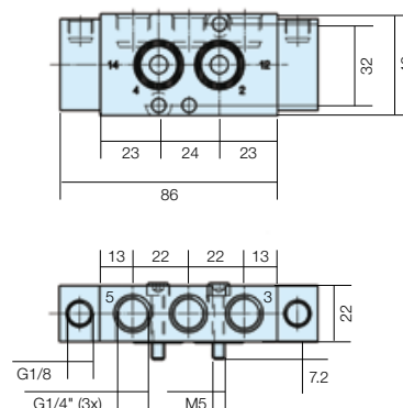
Dimensions Reference 9
