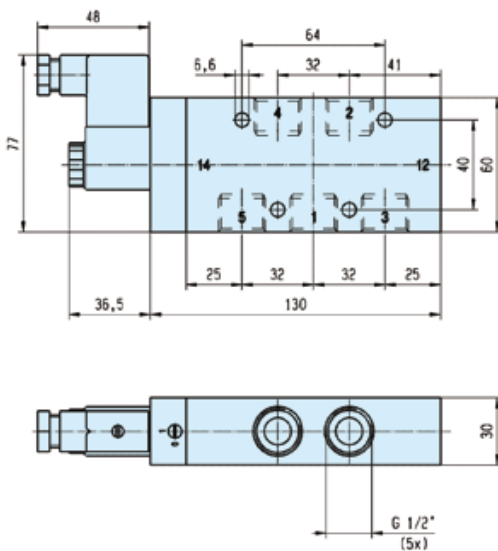
Dimensions Reference 22
