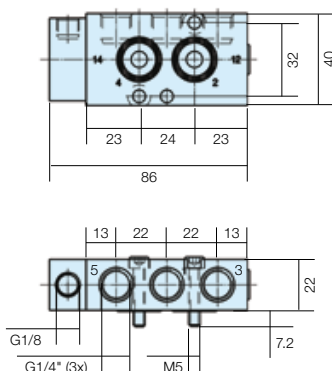
Dimensions Reference 8
