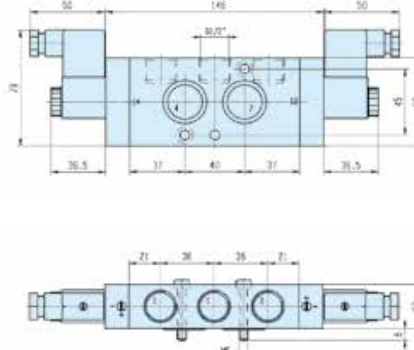
Dimensions Reference 12
