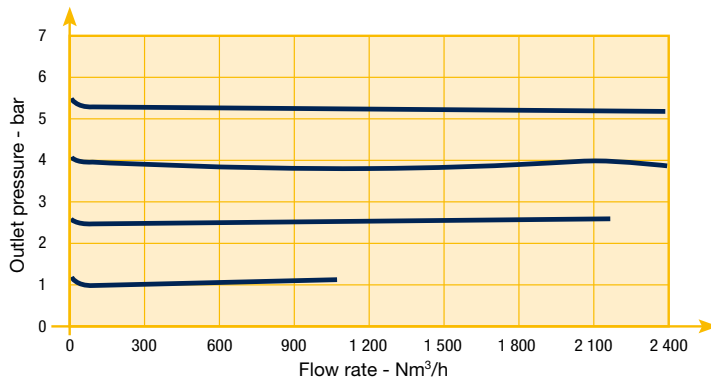
Flow Curve 2"
