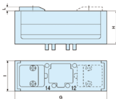
Pneumatically actuated
