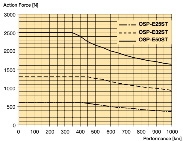
Note: Graph above is based upon 10% intermittent usage
