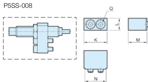
Mounted to table
