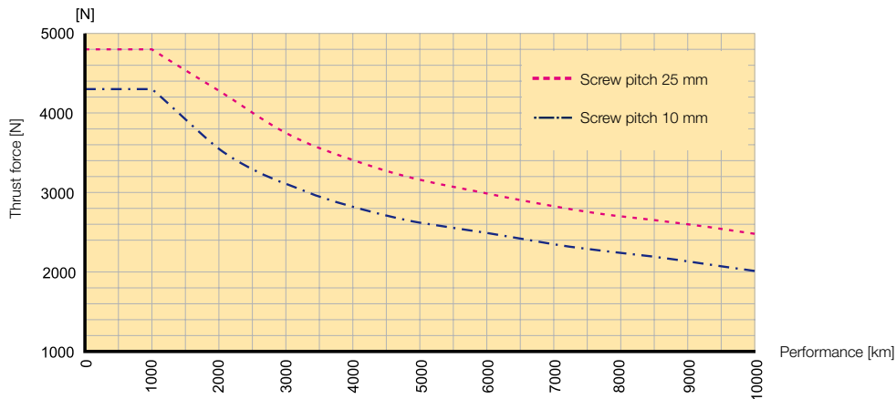
HMRS18 Performance / Thrust force
