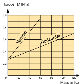
Size OSP-E32SB, Pitch 5mm Acceleration 2 m/s 2
