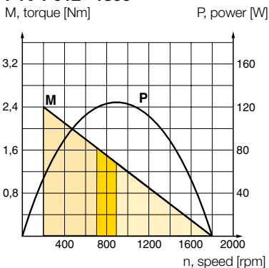
P1V-P012**1800
