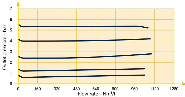
Flow Curve 2"
