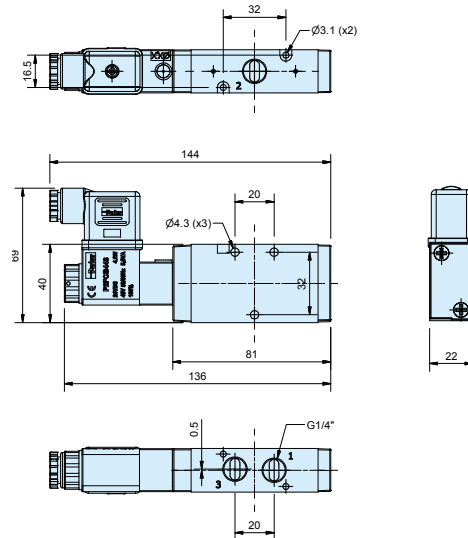
P2LBZ 5/2 Solenoid / Spring
