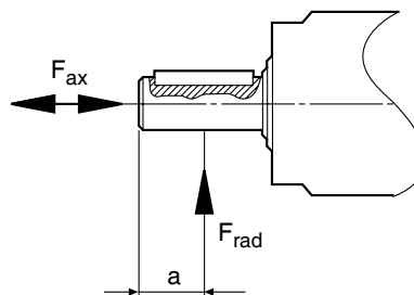
Fig. 1: Loading on output shaft.
