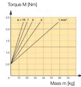
Size OSP-E32B, Horizontal Application
