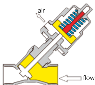
Valve Closed
