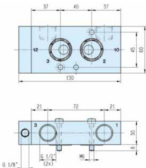
Dimensions Reference 16
