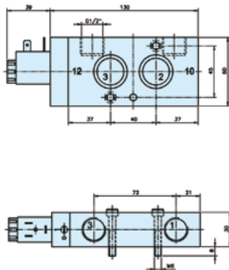
Dimensions Reference 10
