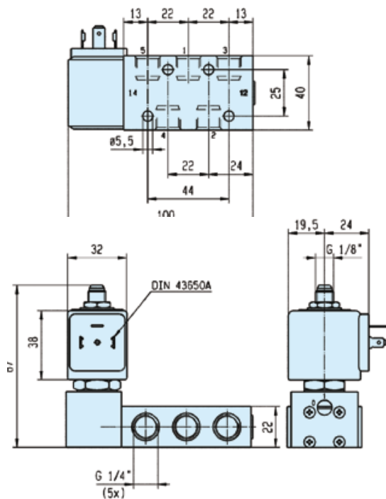
Dimensions Reference 20
