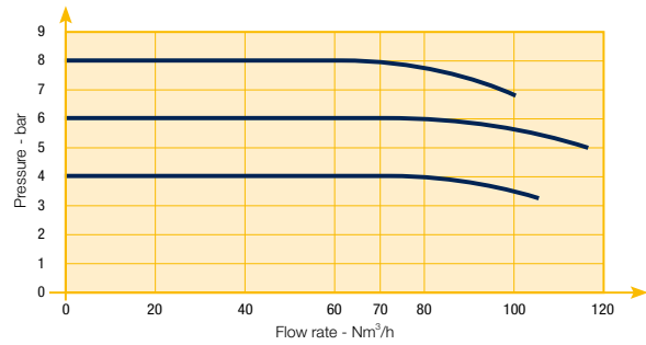
Flow Curve 1/4"
