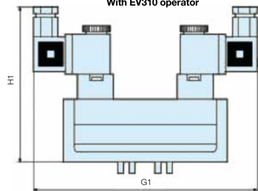
With EV310 operator
