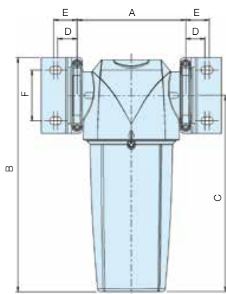
Modular Connection Kit Fixing clamp allows quick and simple connection of multiple filter housings.
