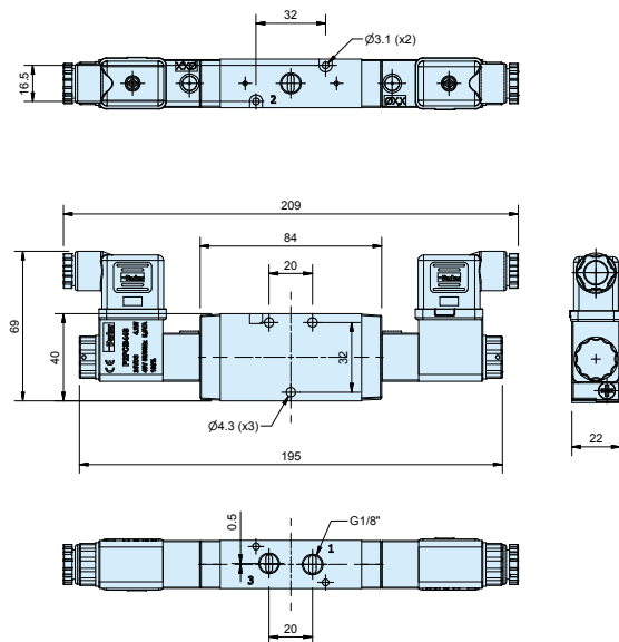
P2LAZ 3/2 Solenoid / Solenoid
