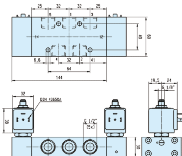
Dimensions Reference 25
