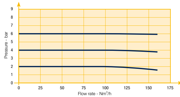
Flow Curve 1/2"
