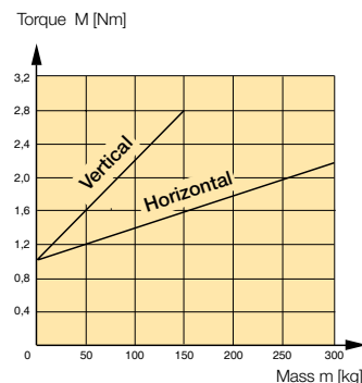
Size OSP-E50SB, Pitch 5mm Acceleration 2 m/s 2
