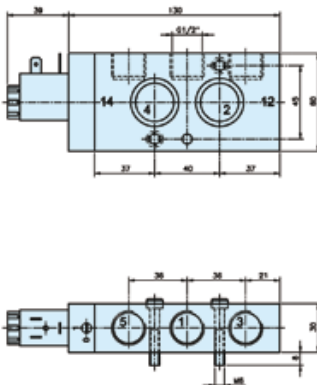
Dimensions Reference 11
