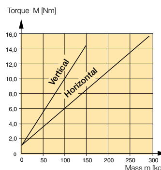
Size OSP-E50SB, Pitch 25mm Acceleration 10 m/s 2
