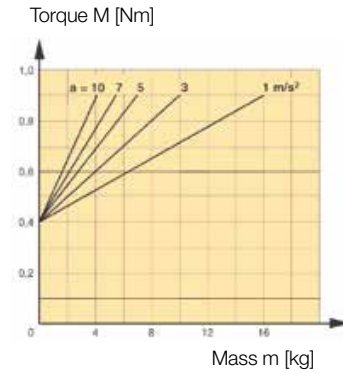
Size OSP-E25B, Horizontal Application
