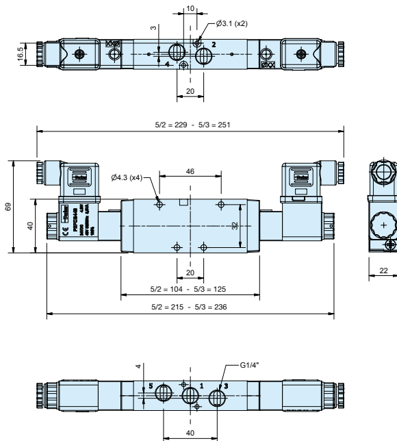
P2LBZ 5/2 and 5/3 Solenoid / Solenoid
