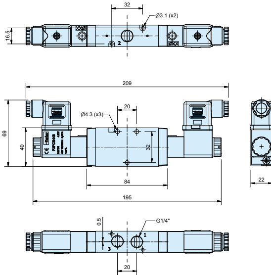
P2LBZ 3/2 Solenoid / Solenoid
