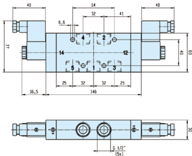
Dimensions Reference 23
