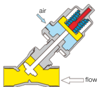
Valve Open
