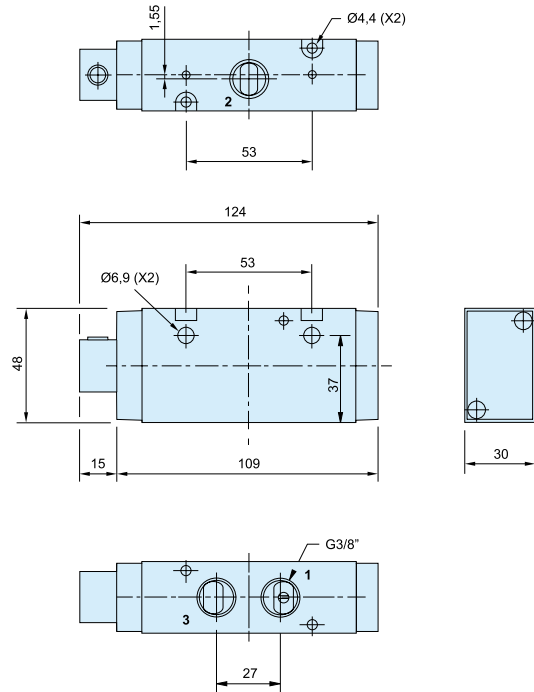
P2LCZ 3/2 Solenoid / Spring
