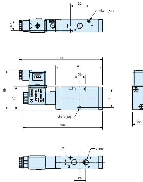
P2LAZ 3/2 Solenoid / Spring
