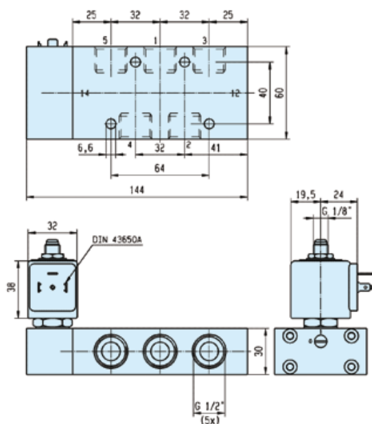
Dimensions Reference 24
