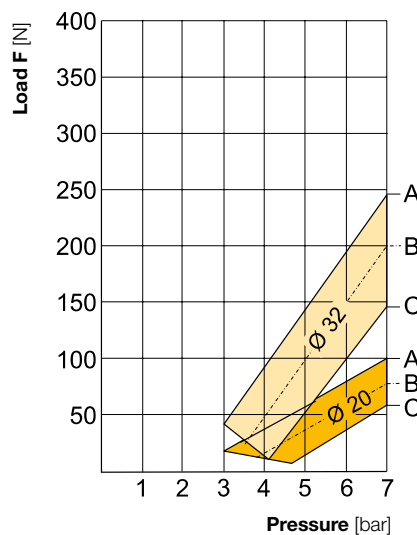
Cylinder Ø 20, 32
