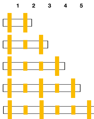
Position of T-Brackets for multiple units
