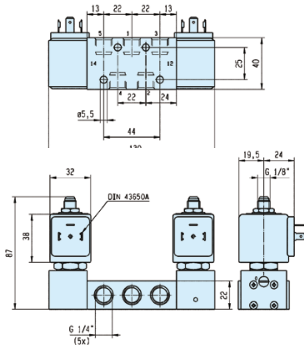
Dimensions Reference 21
