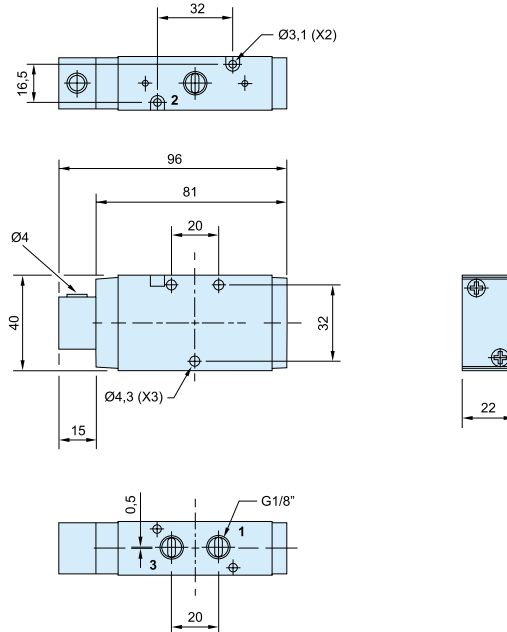
P2LAZ 3/2 Solenoid / Spring
