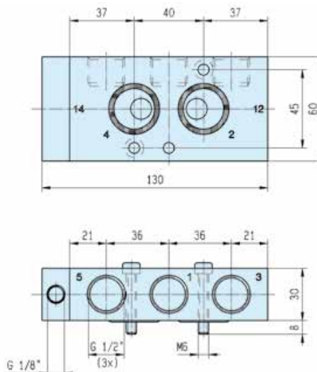
Dimensions Reference 17
