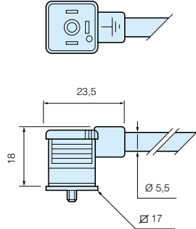
Connector with standard screw
