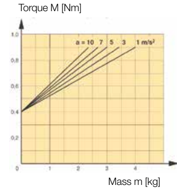
Size OSP-E25B, Vertical Application
