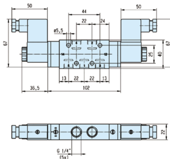
Dimensions Reference 19
