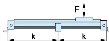
Permissible Unsupported Length STL25 to STL50
