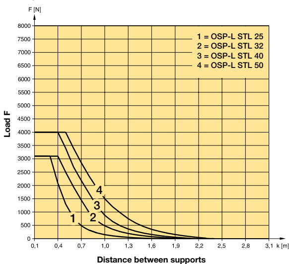
Loading 2 – Side carrier
