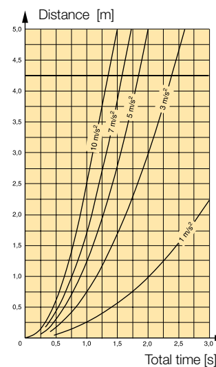
Max speed 5 m/s
