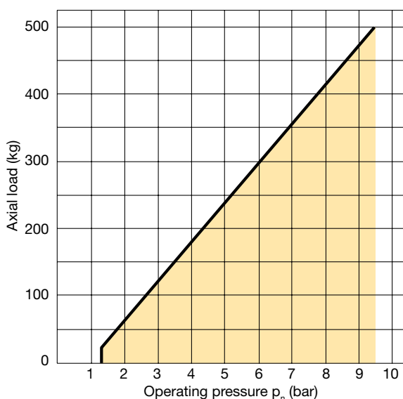
Axial load subject to operating pressure – Type STVSR-80-40
