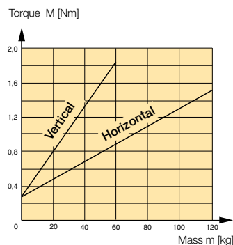
Size OSP-E32SB, Pitch 10mm Acceleration 4 m/s 2
