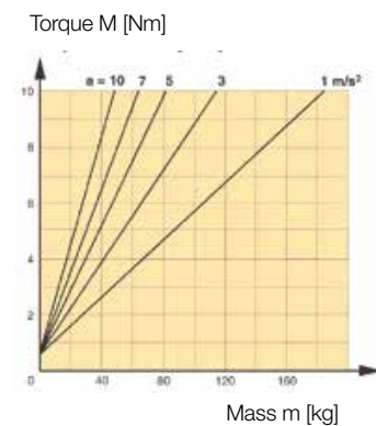
Size OSP-E50B, Horizontal Application
