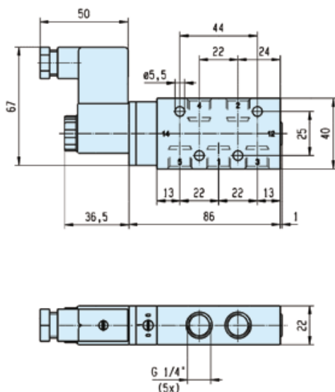
Dimensions Reference 18
