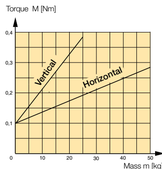
Size OSP-E25SB, Pitch 5mm Acceleration 2 m/s 2
