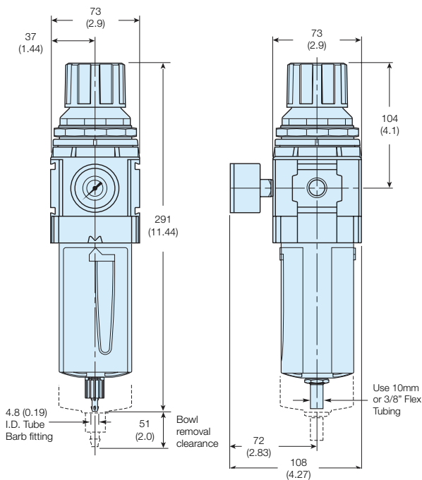
Manual Drain
