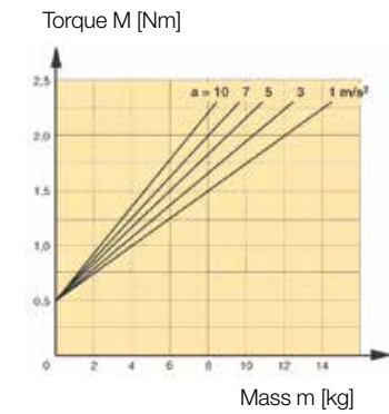
Size OSP-E32B, Vertical Application
