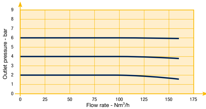
Flow Curve 1"
