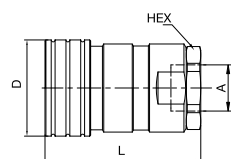
Female Thread
