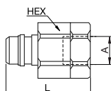
Female Thread
