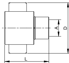
Female Thread
