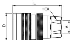
Female Thread
