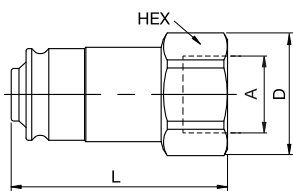
Female Thread*
