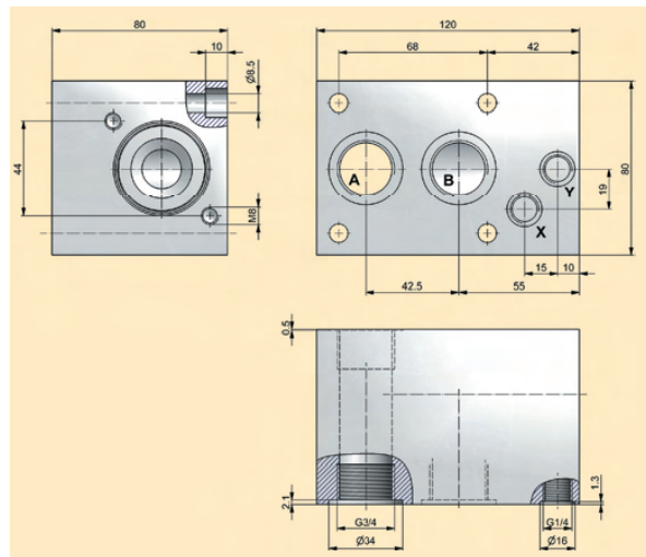
Connection block SCAQ-150
