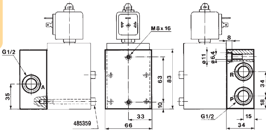
Sub-base 485291
