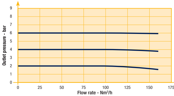
Flow Curve 1"
