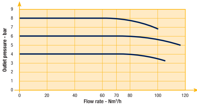
Flow Curve 1/4"
