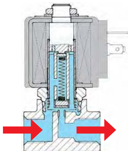
Energised
