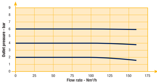
Flow Curve 1/2"
