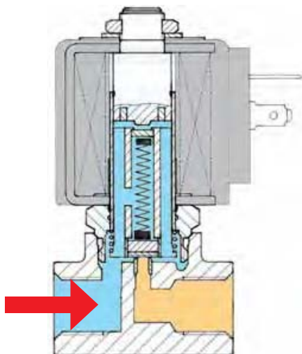
De-energised
