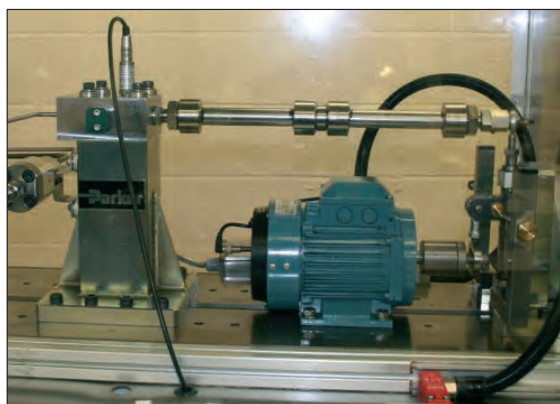
Vibration test
