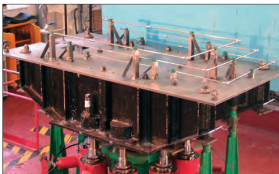
Shock test
