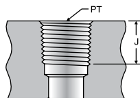
NPTF and BSPT Port
