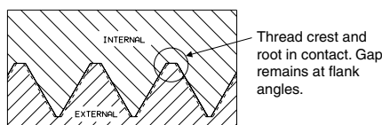
Fig. F2 — NPTF: Hand Tight, Crest to Root Contact
