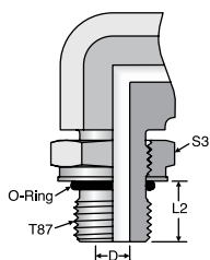
ISO 6149 Adjustable
