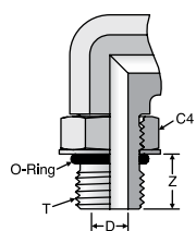
SAE J1926 Adjustable
