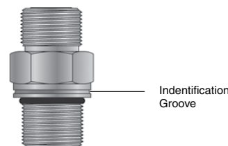
Fig. F7 — ISO 6149 Male
