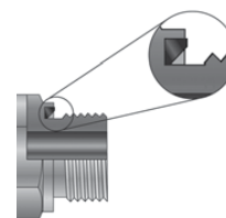
Fig. F6 — O-Ring in Fitting Groove
