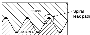
Fig. F1 — NPT: Wrench Tight, No Crest-Root Contact, Flank Contact Only
