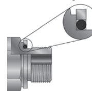
Fig. F5 — O-Ring with Retaining Ring
