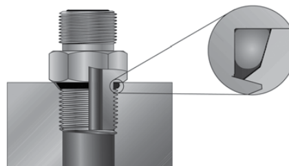
Fig. F4 — Typical O-Ring Boss Port
