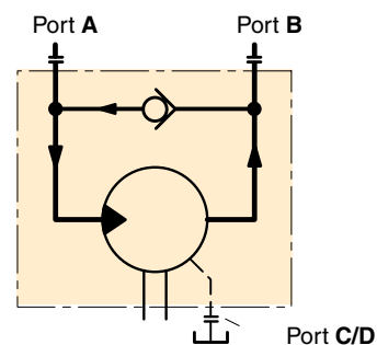
Schematic Fan motor with anti cavitation valve
