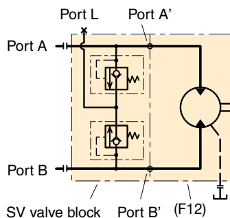
Hydraulic schematic.
