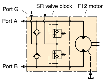
SR valve block schematic.
