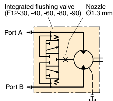
Hydraulic schematic.
