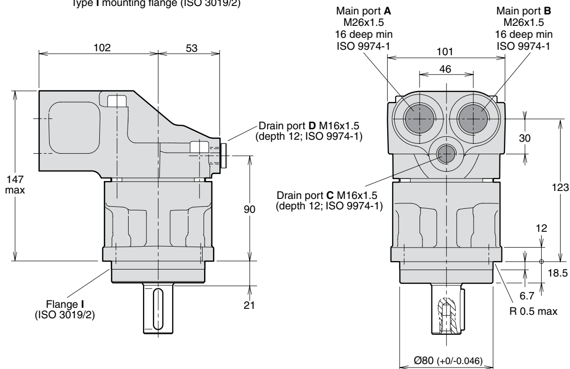
Type I mounting flange (ISO 3019/2)
