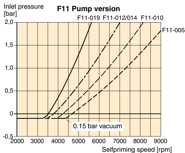
Diagram 2. Min required inlet pressure for Pump.
