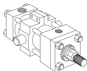
Style DD Intermediate Fixed Trunnion (NFFA Style MT4)
