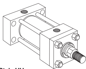
Style HH Rectangular Cap (NFPA Style ME6)
