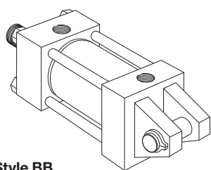
Style BB Cap Fixed Clevis (NFA Style MP1)
