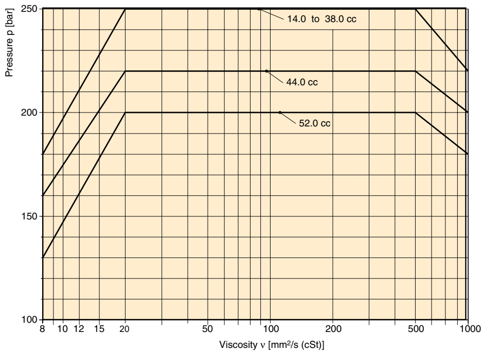
Pressure depending on viscosity
