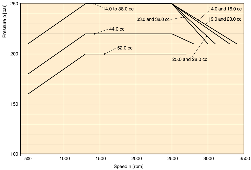
Pressure depending on speed
