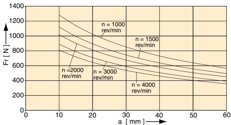
Shaft load for outboard bearings PGP/PGM 511
