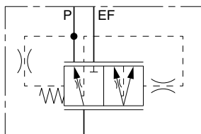
Priority Flow Divider Function "A"
