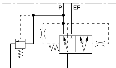
Priority Flow Divider With Full Flow R/V Function "B"
