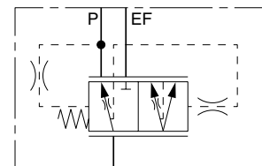
Priority Flow Divider Function "A"
