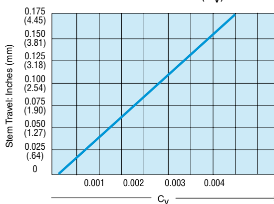
Flow Coefficient ( C_v )
