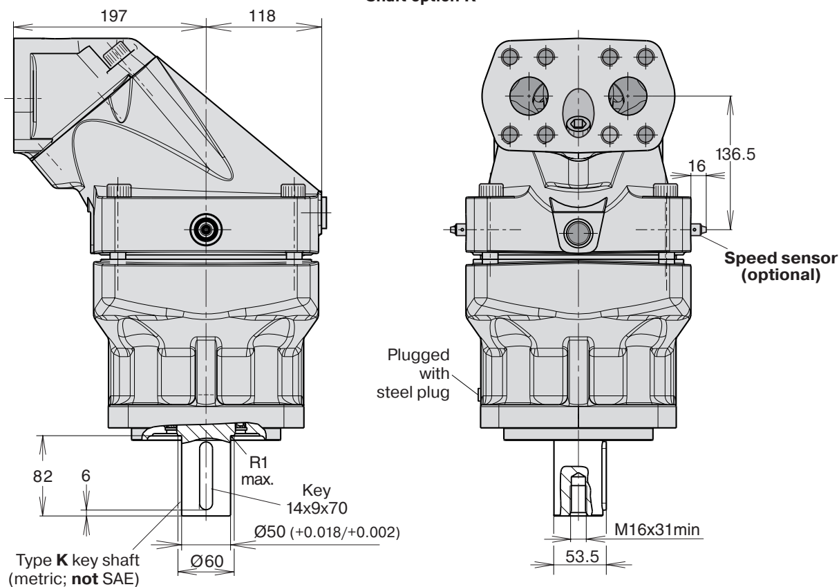
Shaft option K
