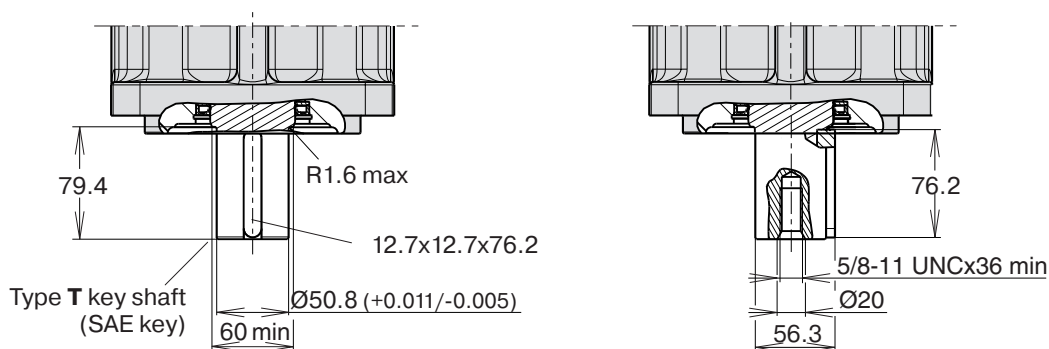
Shaft option T
