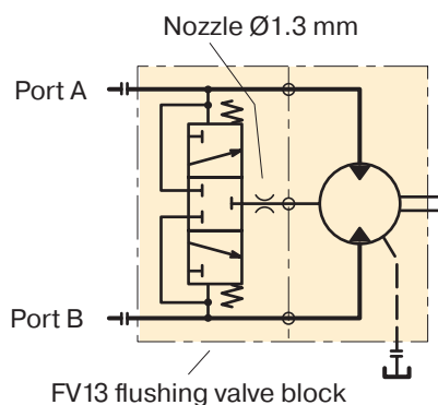
Hydraulic schematic.
