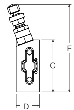
Example shown: 5-valve extruded direct mount manifold with Parker Superior Advantage fully integrated inverted A-LOK® tube fitting connections.
