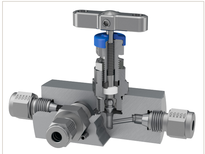
HNV series gauge vent hand valve with inverted tube fitting to inlet and outlet connections with Parker PTFree connect™ tube fitting connection to the vent.
