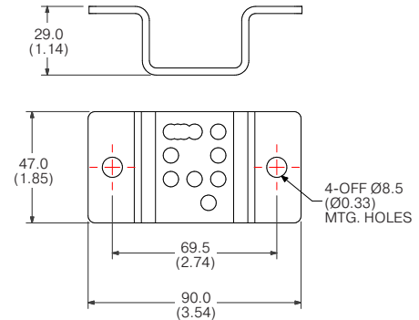
Image shown: Part No.: BKT1SSB1
