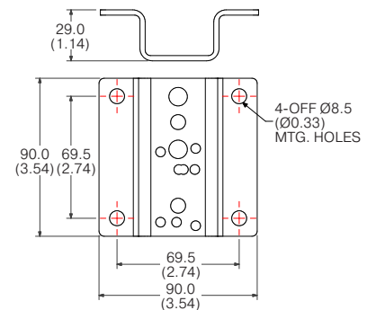
Image shown: Part No.: BKT2SSB2
