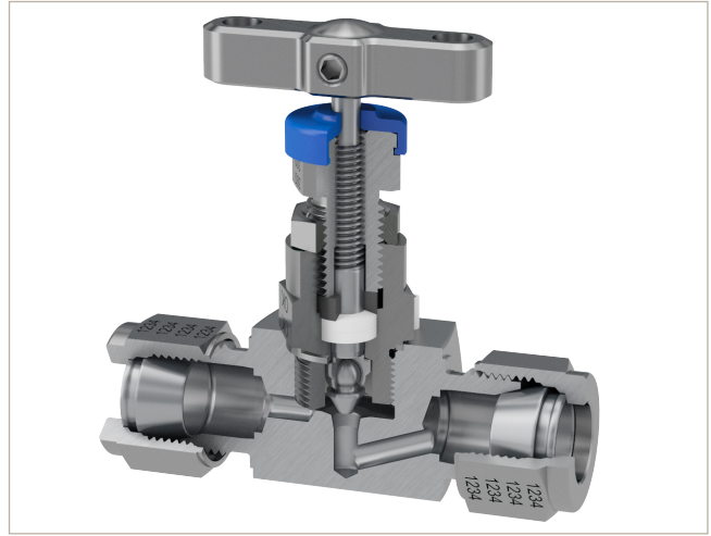
HNV series hand valve with traditional type fully integrated tube fitting connection.
